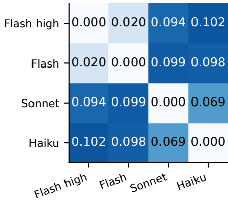
Between-model symbol JS
