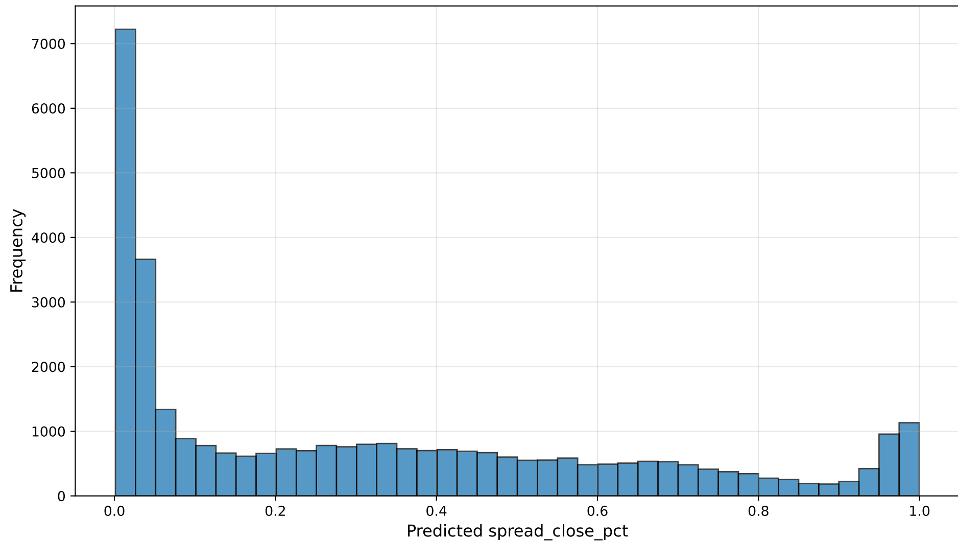
LASSO Linear Classifier - Prediction Distribution
