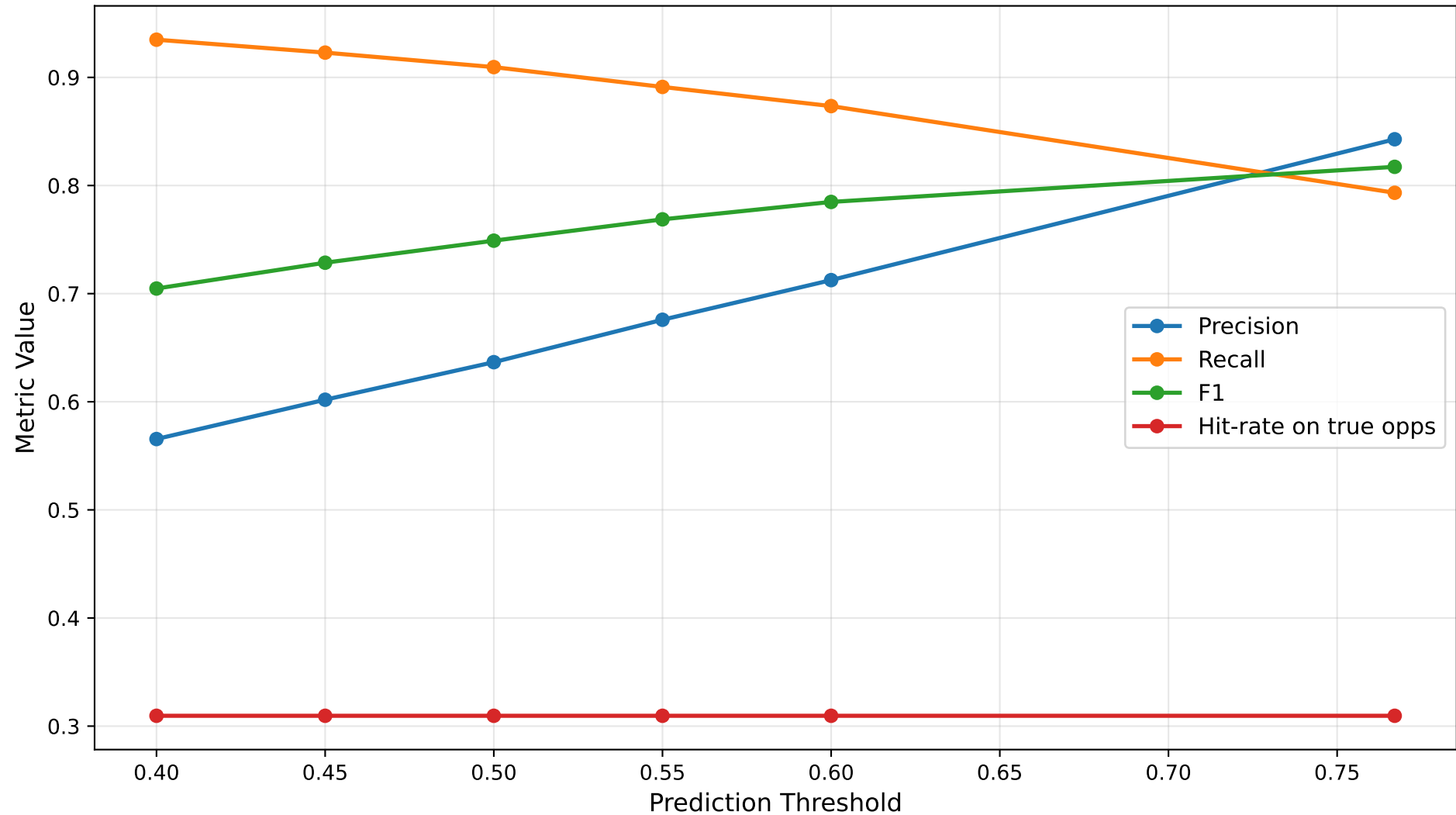
RIDGE Linear Classifier - Threshold Analysis
