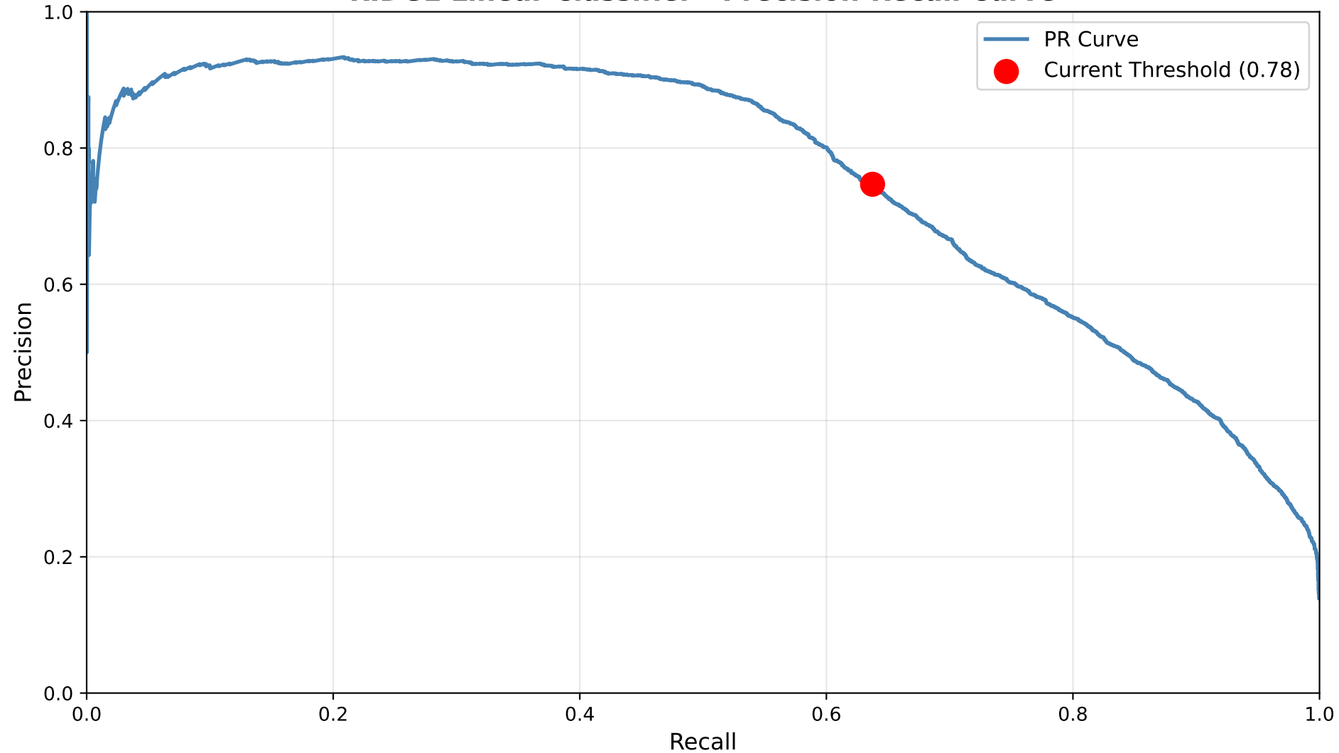
RIDGE Linear Classifier - Precision-Recall Curve
