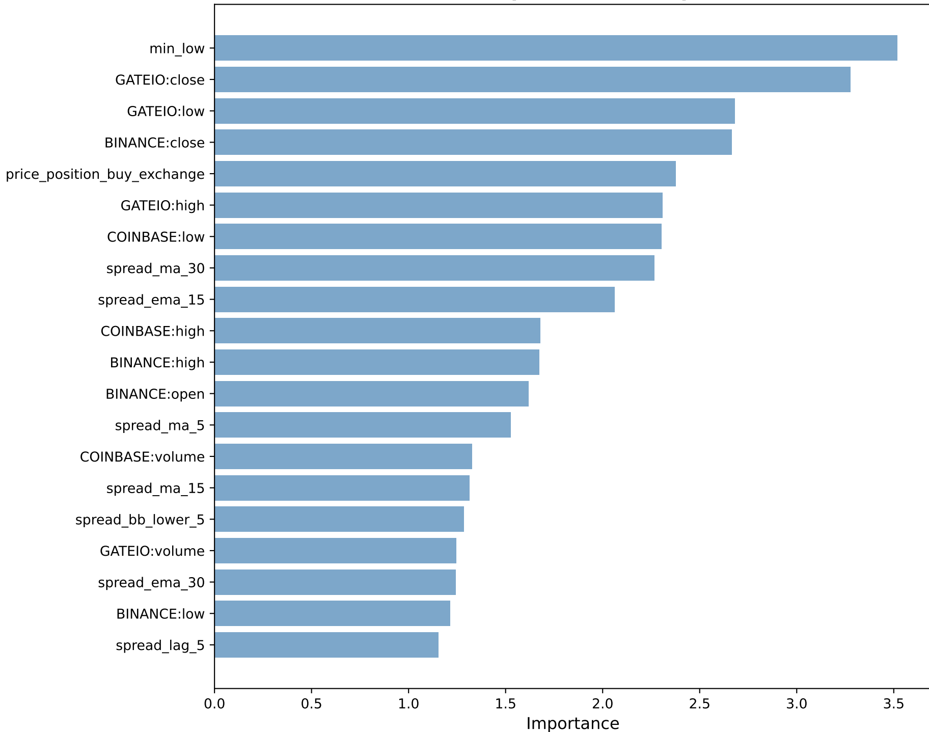
CatBoost- Top 20 Feature Importance
