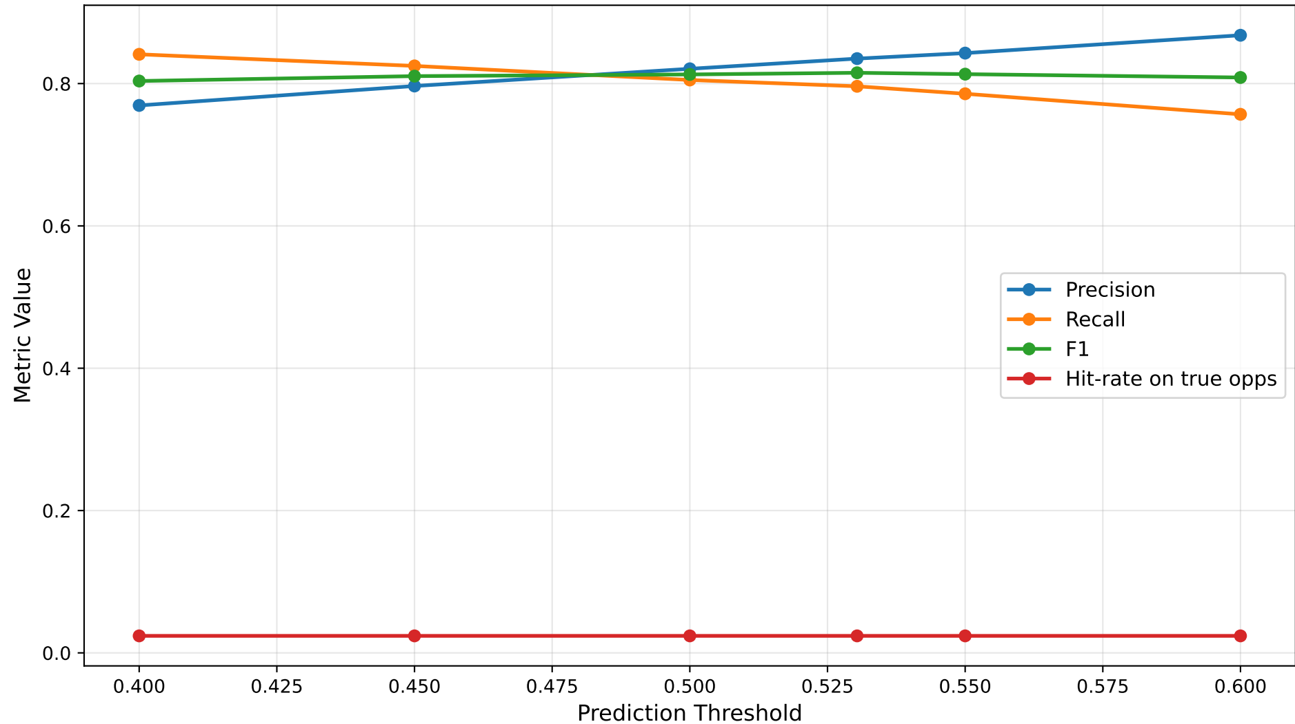
CatBoost - Threshold Analysis
