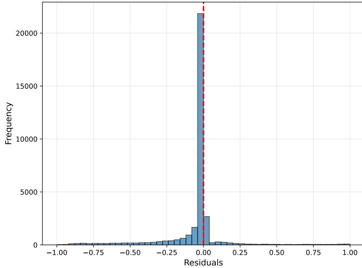
Residual Distribution
