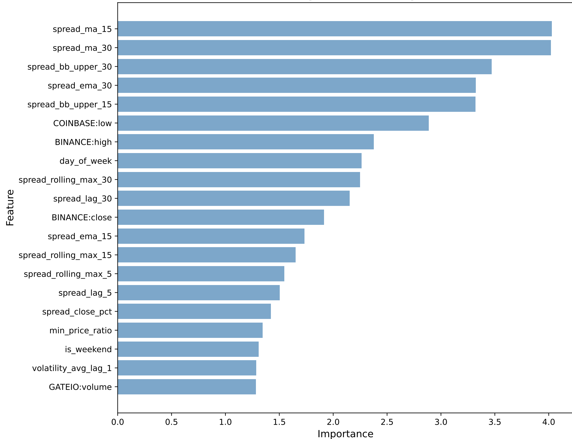
CatBoost - Top 20 Feature Importance
