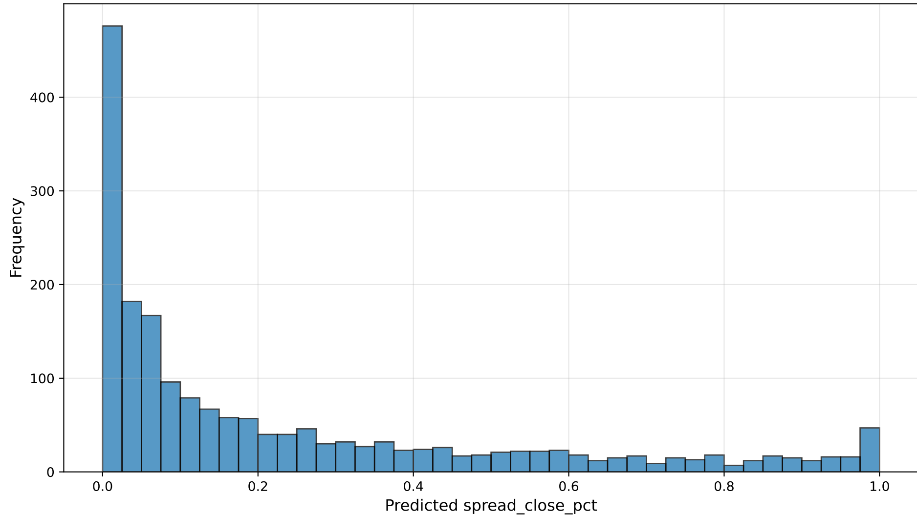
GRU - Prediction Distribution
