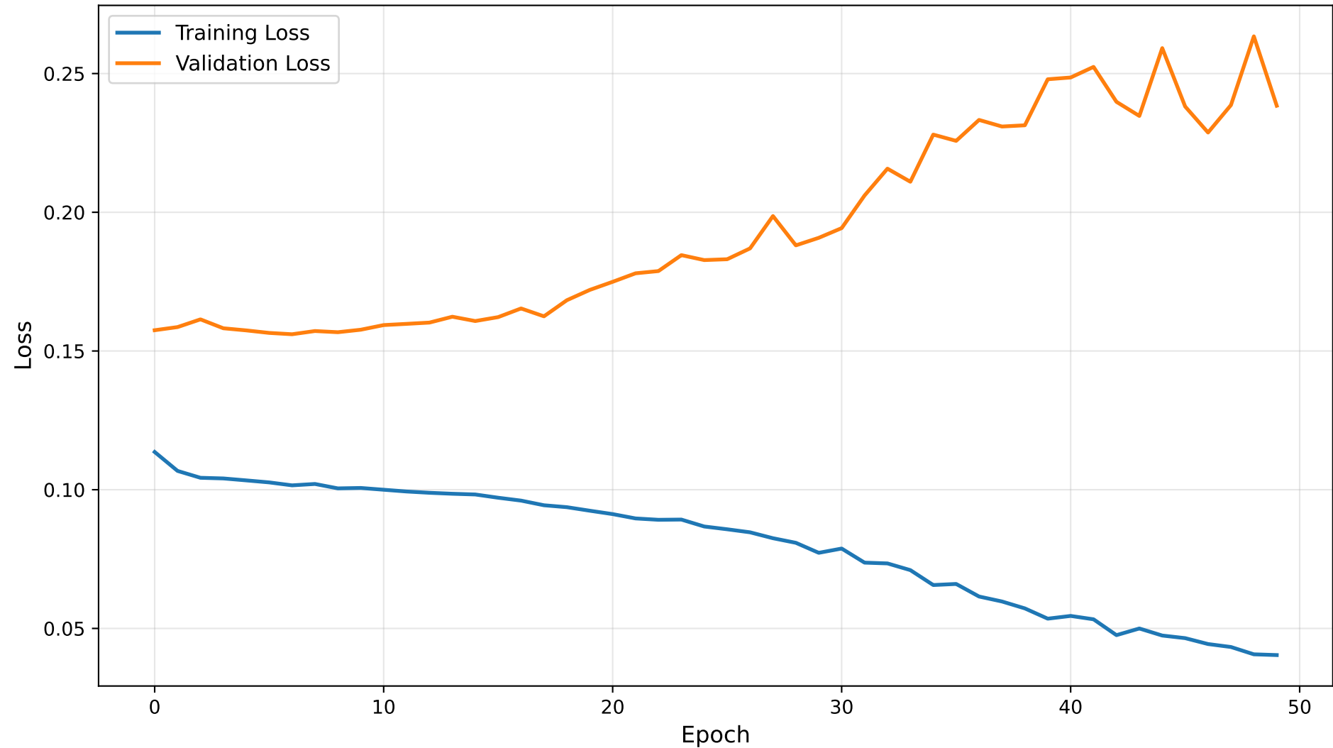
GRU - Training and Validation Loss Over Epochs
