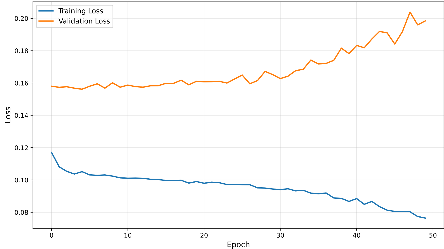
LSTM - Training and Validation Loss Over Epochs
