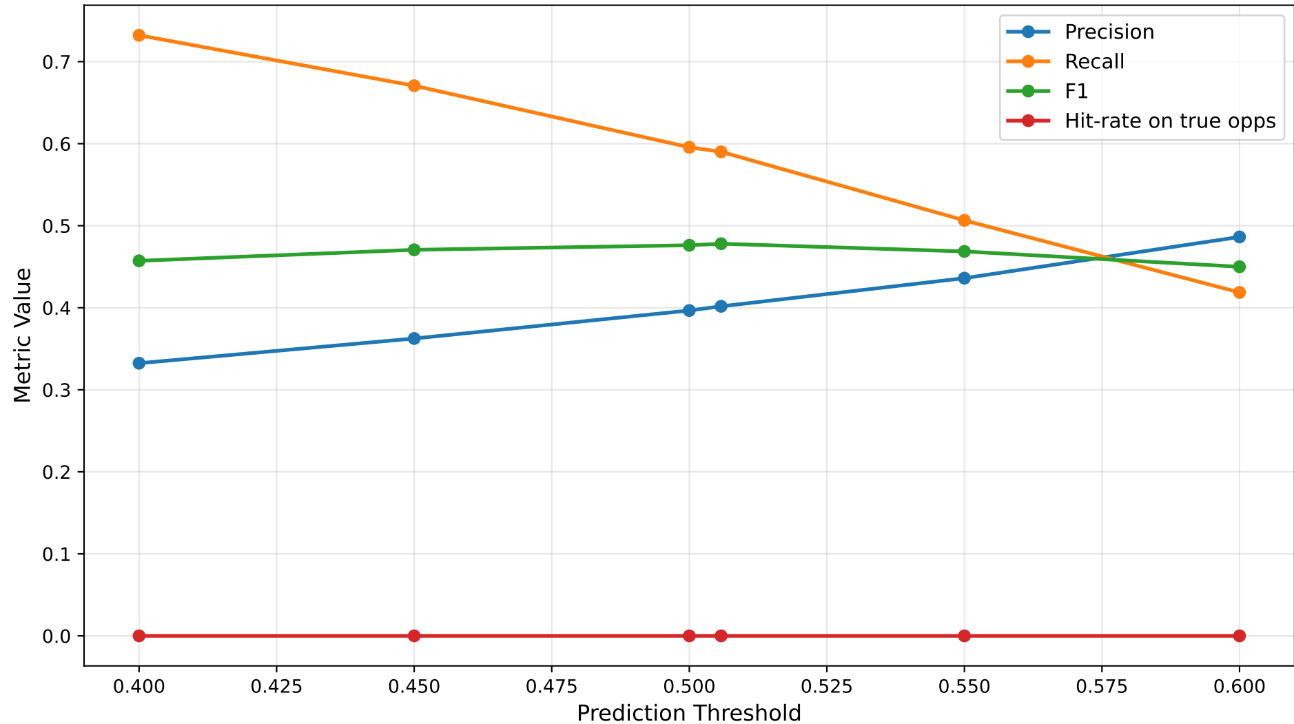
Random Forest - Threshold Analysis
