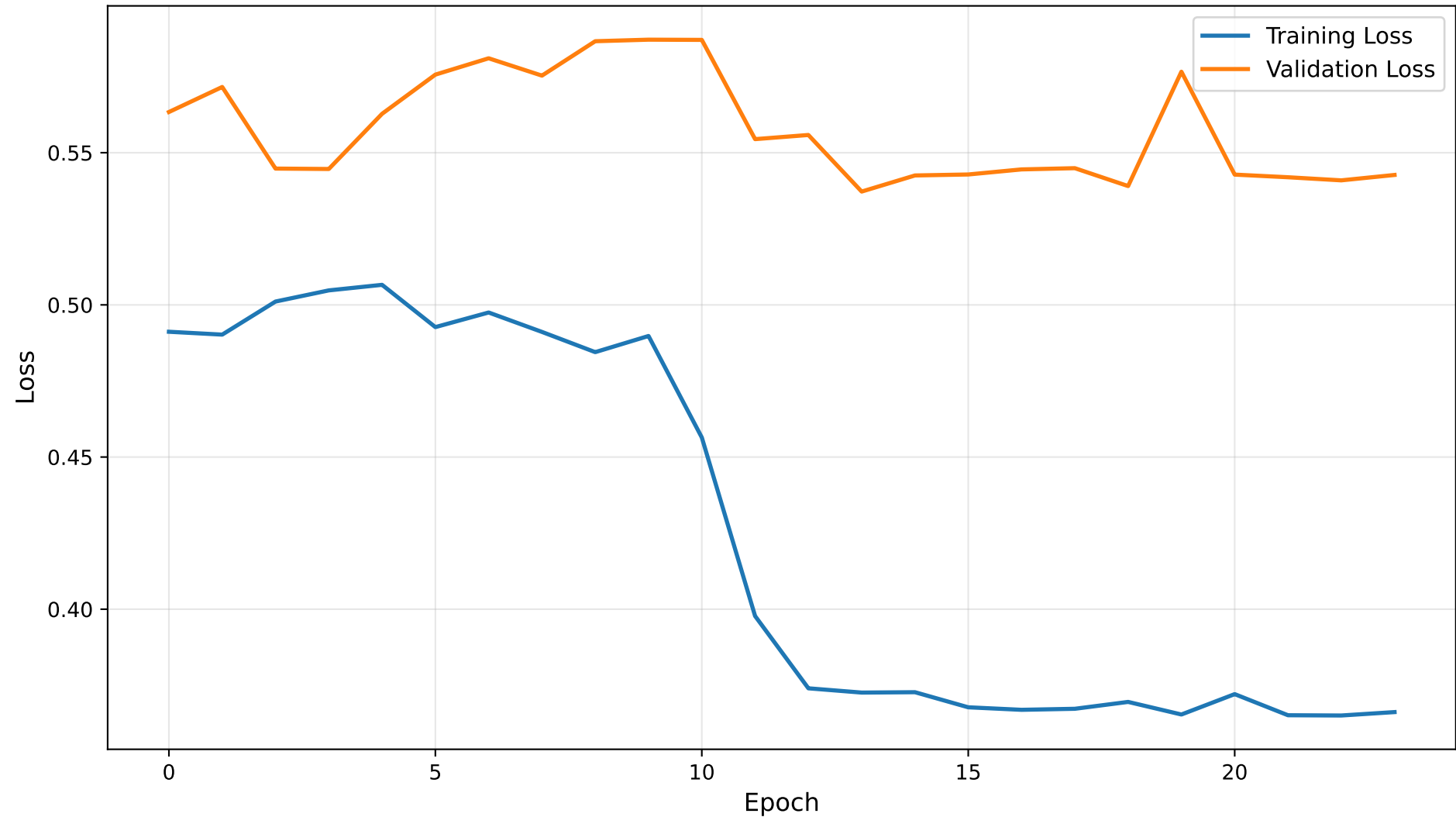
Transformer - Training and Validation Loss Over Epochs
