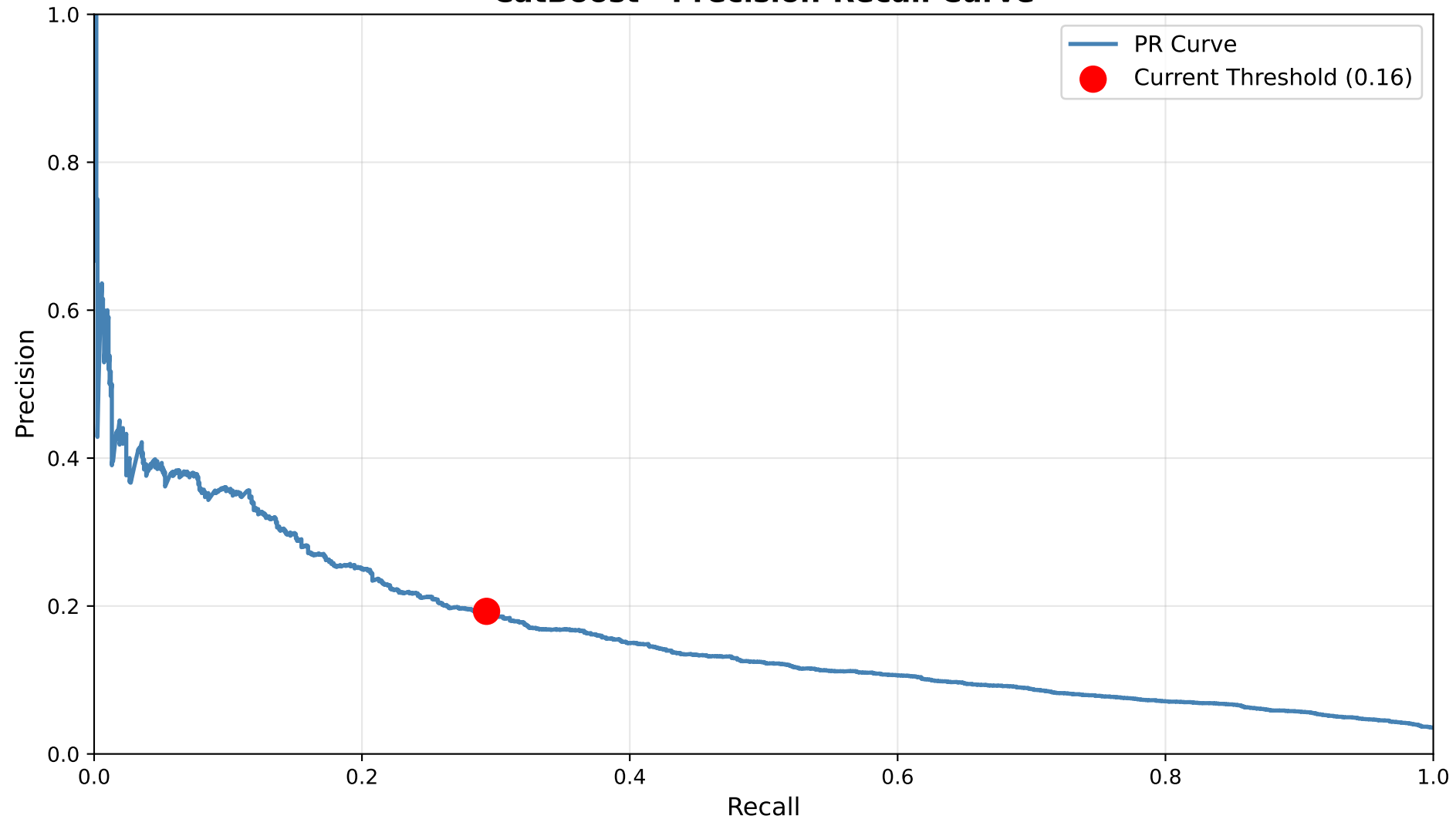
CatBoost - Precision-Recall Curve
