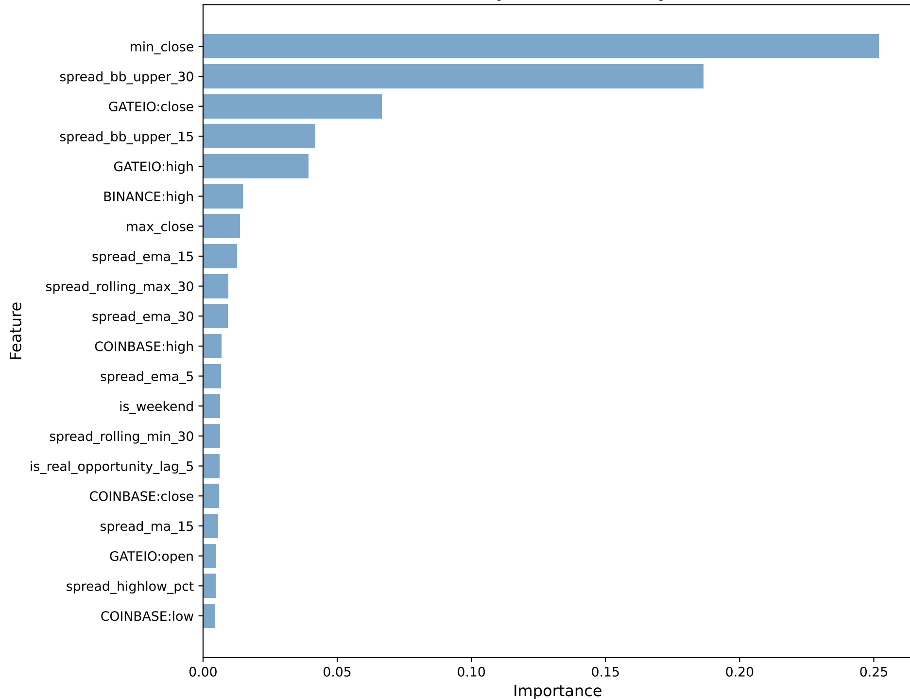
XGBoost - Top 20 Feature Importance
