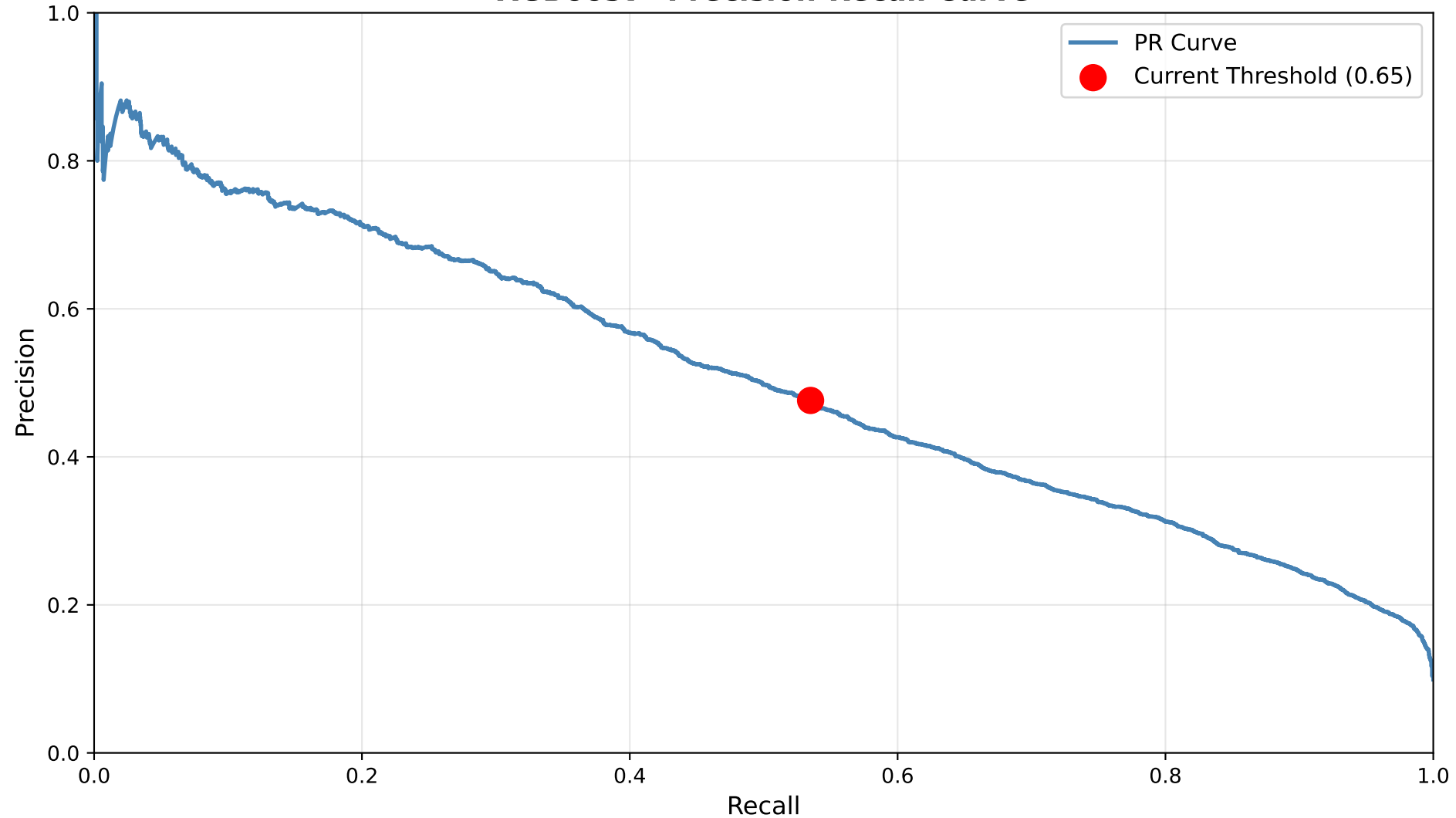
XGBoost - Precision-Recall Curve
