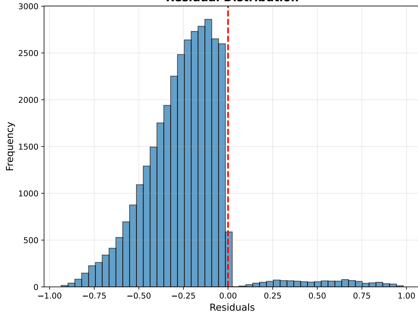
Residual Distribution
