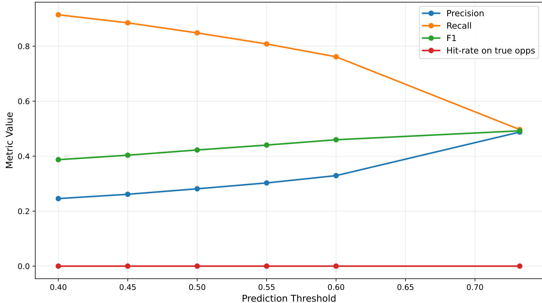
Random Forest - Threshold Analysis
