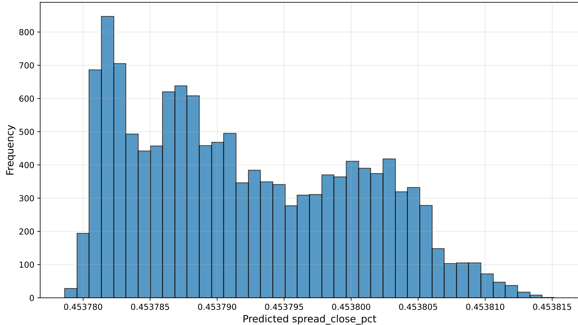
Transformer - Prediction Distribution
