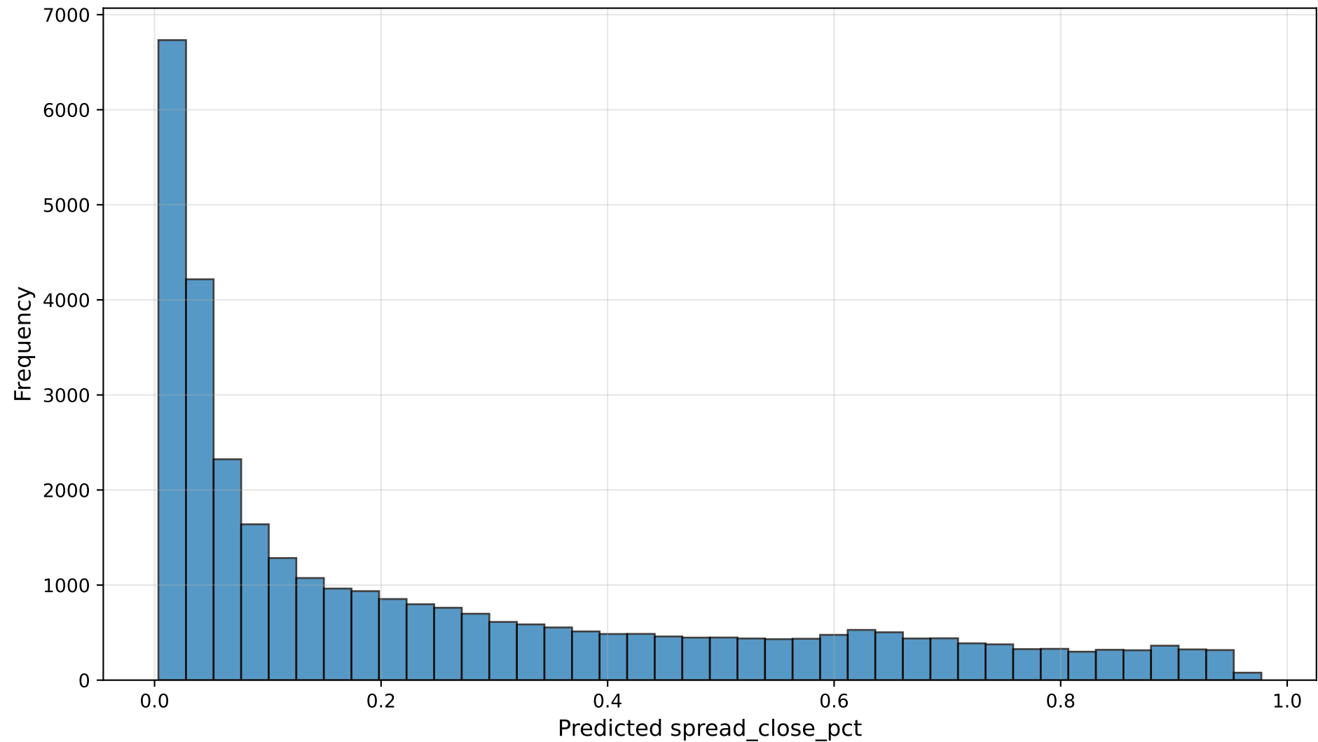
XGBoost - Prediction Distribution
