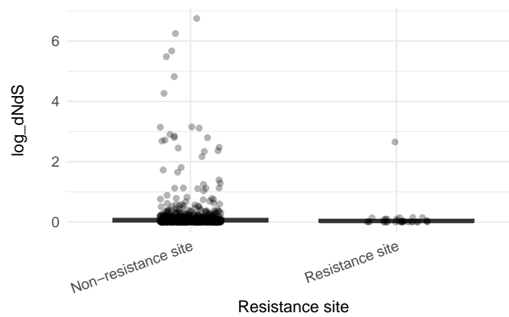
Boxplot of log_dNdS
