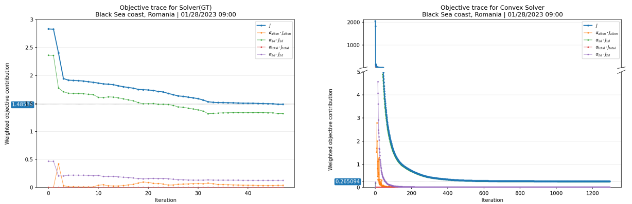
Figure 7: Evolution of the weighted objective over L-BFGS-B iterations for Case Study I. Left: \text{SOLVER}(\text{GT}) , initialized from the ground-truth field, converges to final J = 1.485 . Right: CONVEX SOLVER reaches a lower final weighted objective, J = 0.265 , but its reconstruction is farther from the ground truth by RMSE.
