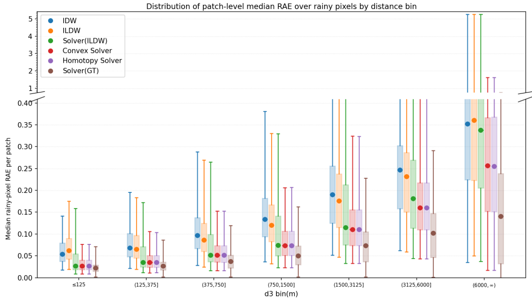
Figure 4: Rainy-pixel d_3 -profile box-and-whisker summary. Each patch contributes one median rainy-pixel relative absolute error value per d_3 bin. Across patches, each box spans the 25th to 75th percentiles, and the whiskers show the minimum and maximum values. The corresponding rainy-pixel counts per bin are reported in Table 4.
