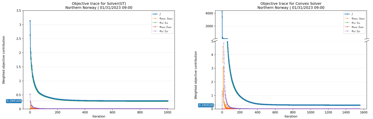
Figure 9: Evolution of the weighted objective over L-BFGS-B iterations for Case Study II. Left: SOLVER(GT), initialized from the ground-truth field, converges to final J = 0.289 . Right: CONVEX SOLVER reaches a very similar final weighted objective, J = 0.290 , and a similar RMSE.
