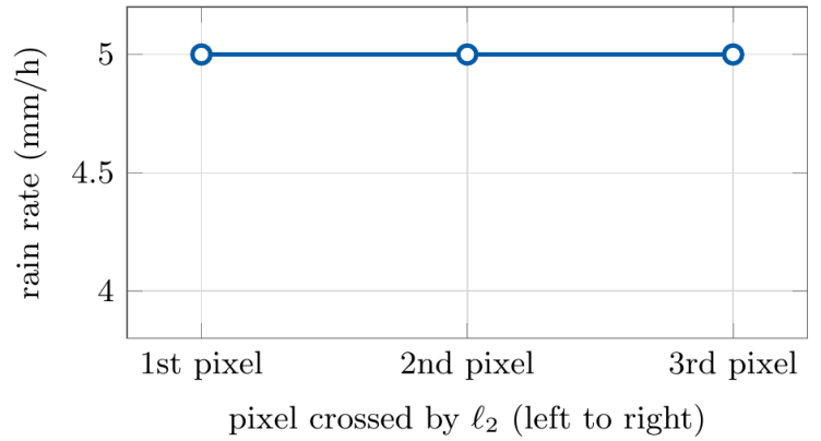
Figure 10: Geometric difference between midpoint IDW and ILDW. Away from the middle column, IDW mixes the 5 \text{ mm h}^{-1} observation from \ell_2 with the neighboring 4 \text{ mm h}^{-1} observation. ILDW associates each link-level observation with every pixel crossed by its segment and therefore exactly recovers this row-wise constant field.
