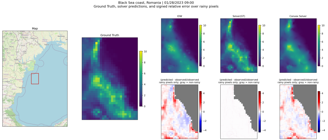
Figure 6: Case Study I: \text{SOLVER}(\text{GT}) is visually close to the ground truth. The three upper-right panels show the rainfall fields reconstructed by IDW, \text{SOLVER}(\text{GT}) , and CONVEX SOLVER. The corresponding lower-right panels show the relative error of each reconstruction.
