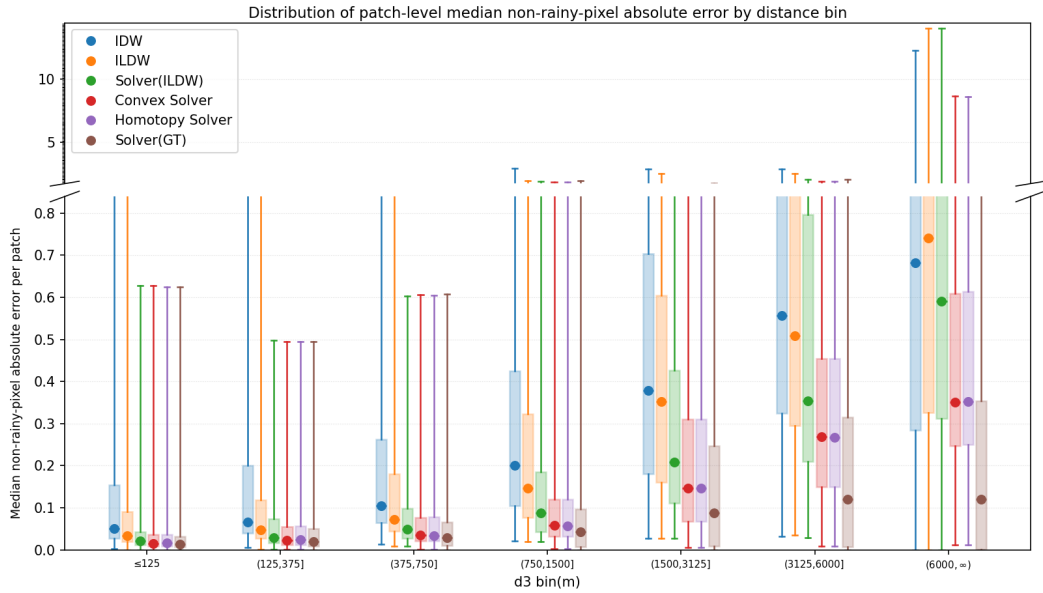
Figure 5: Non-rainy-pixel d_3 -profile box-and-whisker summary. Each patch contributes one median non-rainy-pixel absolute error value per d_3 bin. Across patches, each box spans the 25th to 75th percentiles, and the whiskers show the minimum and maximum values. The corresponding non-rainy-pixel counts per bin are reported in Table 4.
