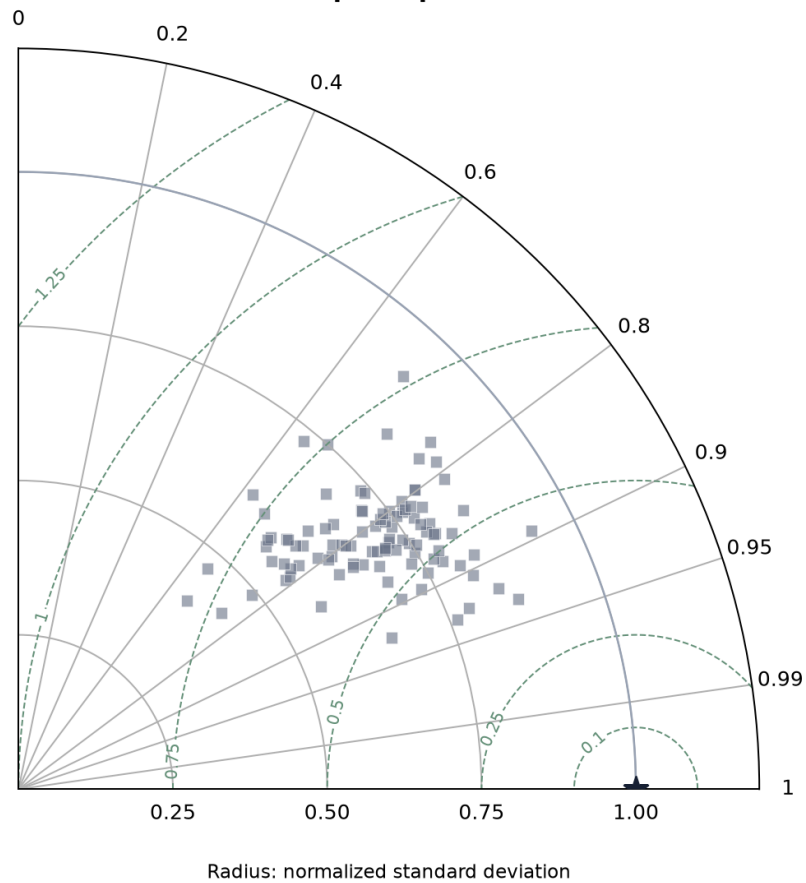
Taylor diagram: IDW 100 patch points
