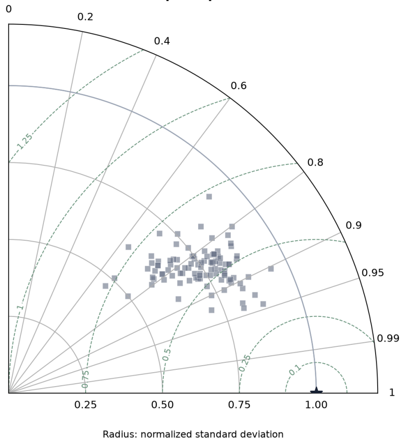
Taylor diagram: ILDW-init Roy DCT 100 patch points
