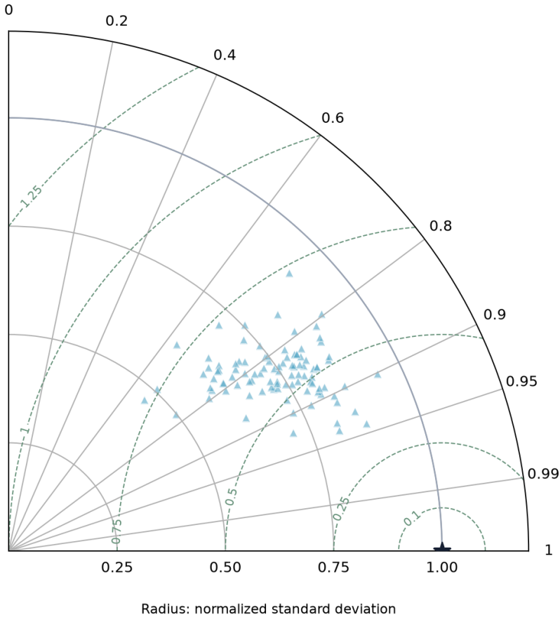
Taylor diagram: ILDW 100 patch points
