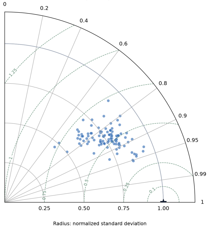
Taylor diagram: Solver(ILDW) no shrinkage 100 patch points
