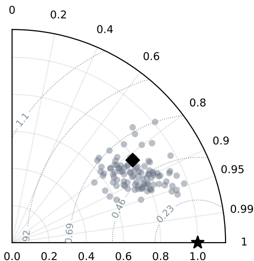
Solver(ILDW)
