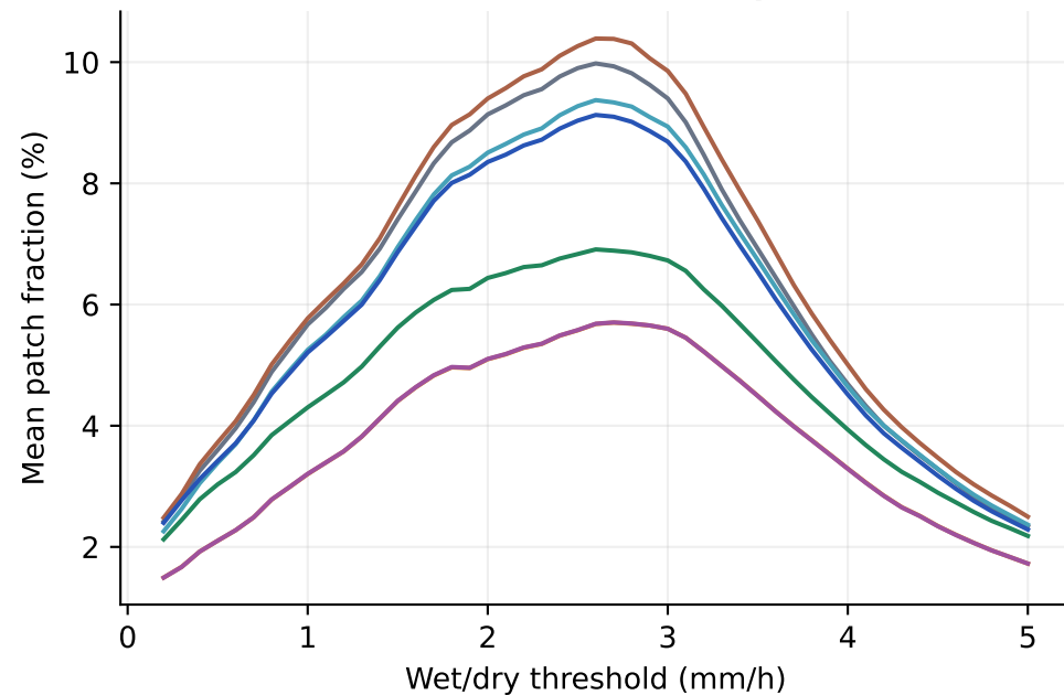
False wet: fraction of all pixels
