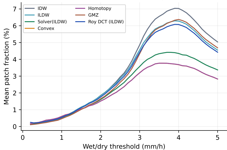
Missed wet: fraction of all pixels
