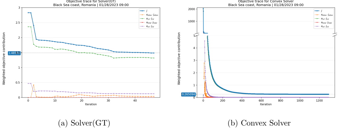
Figure 8: Solver-specific objective traces for the Black Sea coast, Romania case study. Values can be compared over iterations within each panel, but not directly between panels because the solvers use different link models and objective normalizations.
