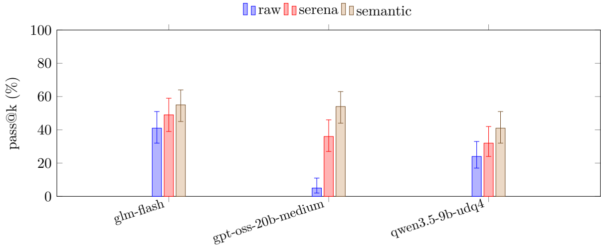
Figure 1: Pass@k by mode, per model. Error bars are 95% Wilson intervals over the k episodes per cell. The ordering \text{semantic} \geq \text{serena} \geq \text{raw} holds for every model in the grid, though at this k the intervals overlap within a model. The lift is largest where the model is a weak freeform tool-caller (gpt-oss-20b-medium at 5% raw, 54% semantic). Generated from committed episode evidence.
