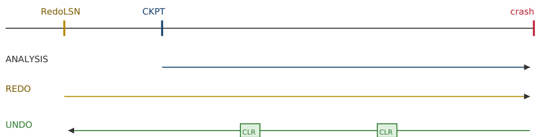
Figure 60.1: the three passes. Analysis scans from the checkpoint to find losers and the RedoLSN; redo scans from the RedoLSN forward, repeating all history; undo scans backward, reversing only losers and logging a compensation record (CLR) for each undo so undo is itself redoable and restartable.
