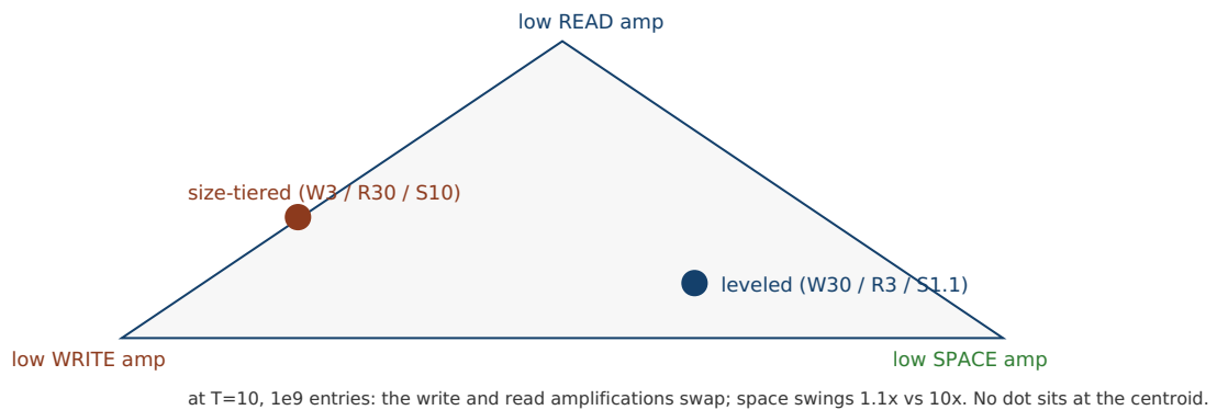
Figure 54.1: the read/write/space trilemma (the RUM tension). Leveled compaction sits near low read and low space, paying high write amplification; size-tiered sits near low write, paying high read and space. The modeled numbers at size ratio T=10 (leveled 30/3/1.1, size-tiered 3/30/10) show the columns swapping — no compaction policy occupies the center where all three are small.
