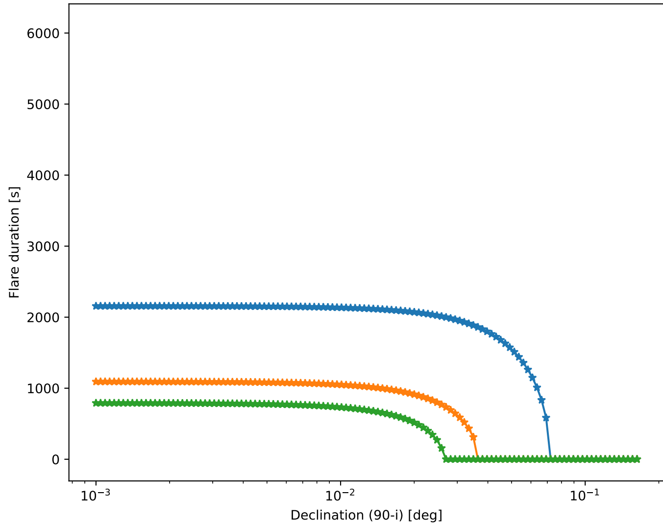
semimajor_axis = 0.3275
