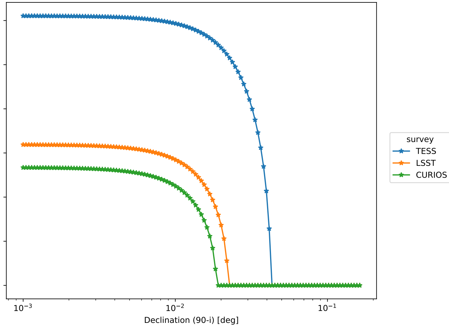
semimajor_axis = 0.9326
