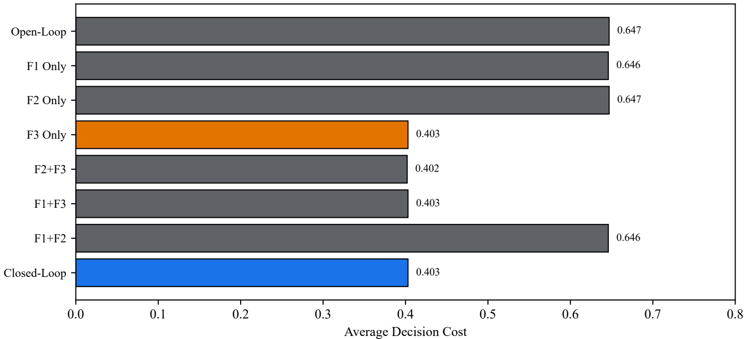
Ablation Study (Rapid Drift, Fixed Cost 10:1)
