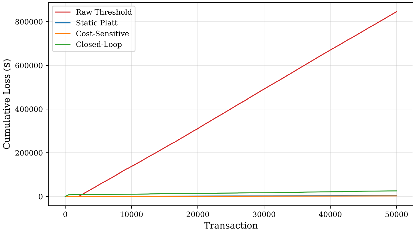
Cumulative Fraud Loss: Closed-Loop vs Baselines
