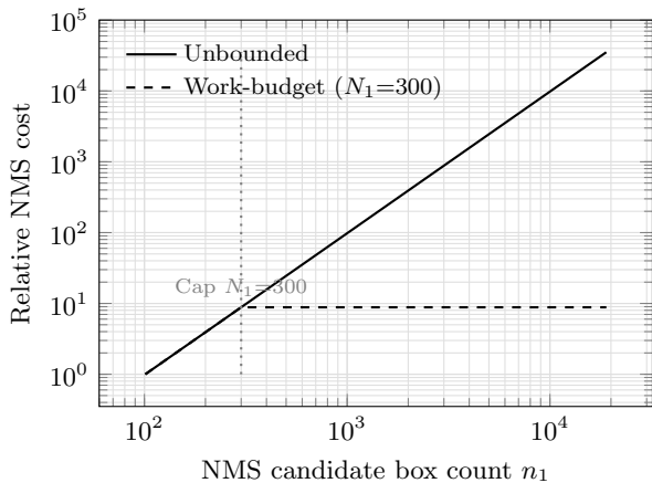
(a) Perception — NMS box flooding
