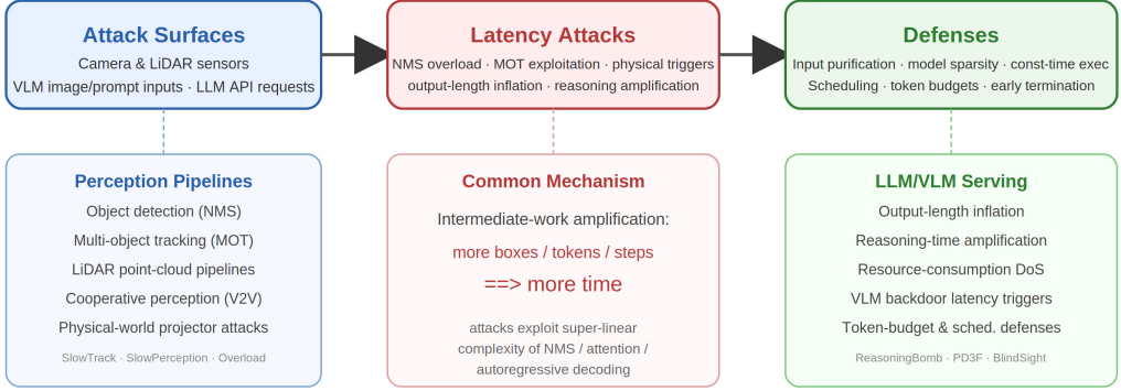
Fig. 2. The intermediate-work amplification principle unifies latency attacks across domains. Attack surfaces (left) feed attacks (center) that succeed by forcing more intermediate objects—boxes, tokens, or reasoning steps—through super-linear-complexity stages, which defenses (right) counter at different intervention layers. The bottom row contrasts the perception-pipeline and LLM/VLM-serving instantiations of the same mechanism.
