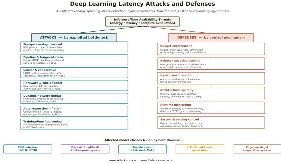
Fig. 1. Overview taxonomy of deep learning latency attacks and defenses. Attacks (left) are organized by the exploited computational bottleneck; defenses (right) by their control mechanism. The bottom band lists the model classes and deployment domains affected. The same content is provided as an editable slide.
