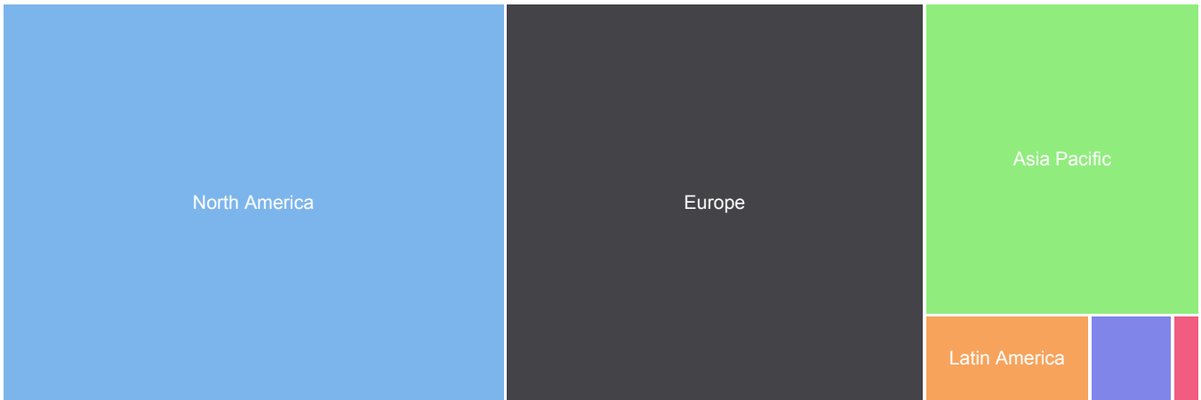
Treemap Chart
