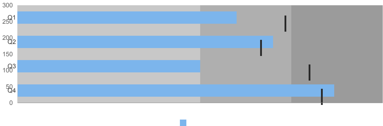
Bullet Chart
