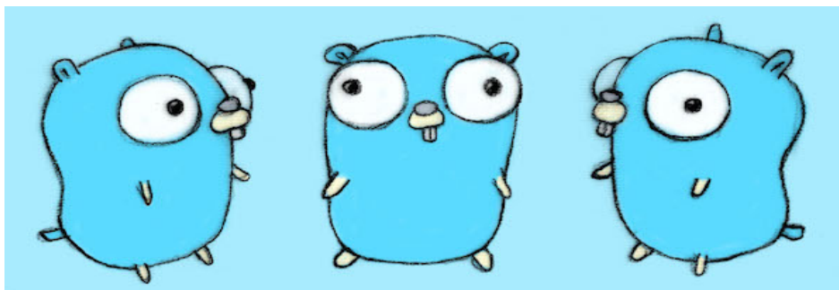
Running Gopher
