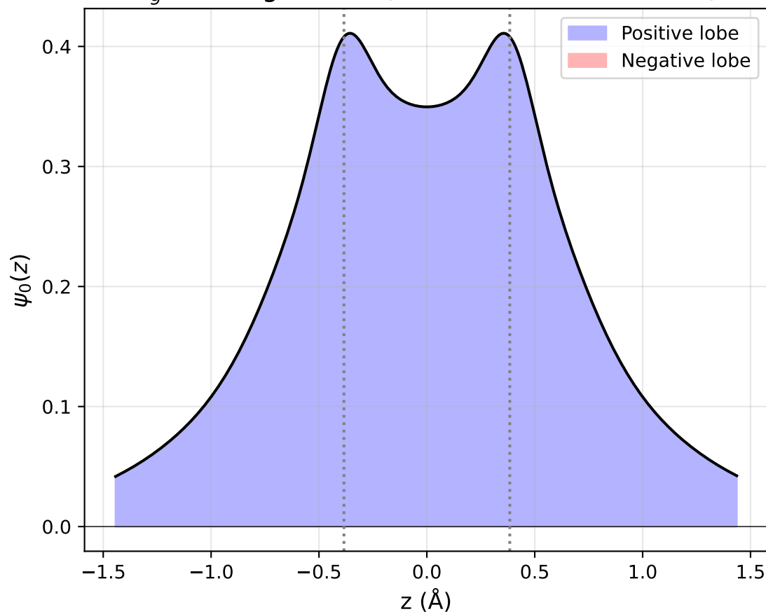
\sigma_g Bonding Orbital (no node between nuclei)
