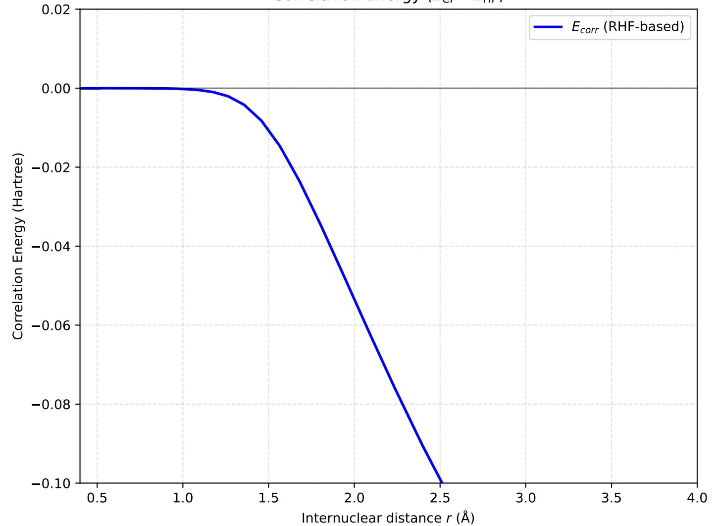
Correlation Energy ( E_{CI} - E_{HF} )
