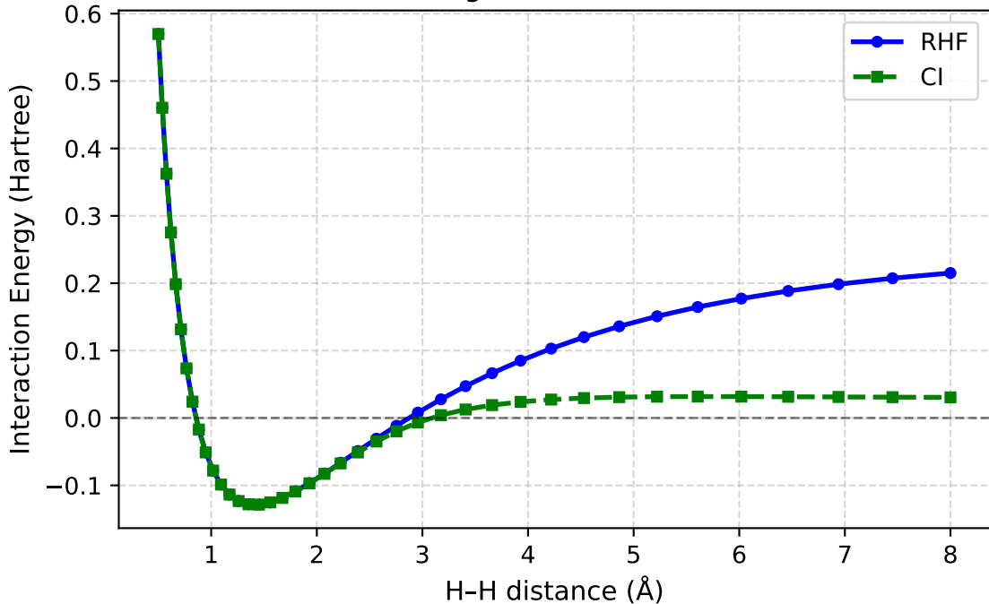
H 2 Binding Curve: E(\text{H}_2) - 2E(\text{H})
