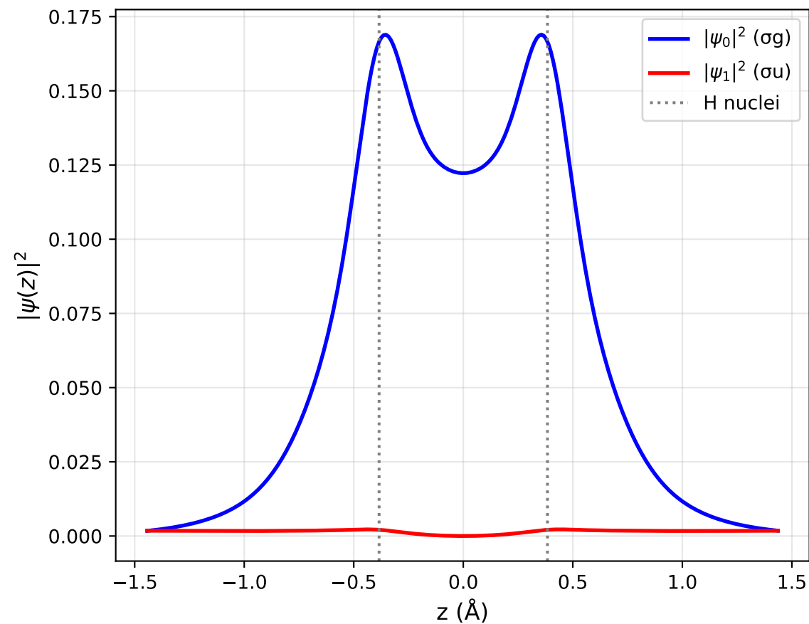
\sigma_u Antibonding Orbital (node at midpoint)
