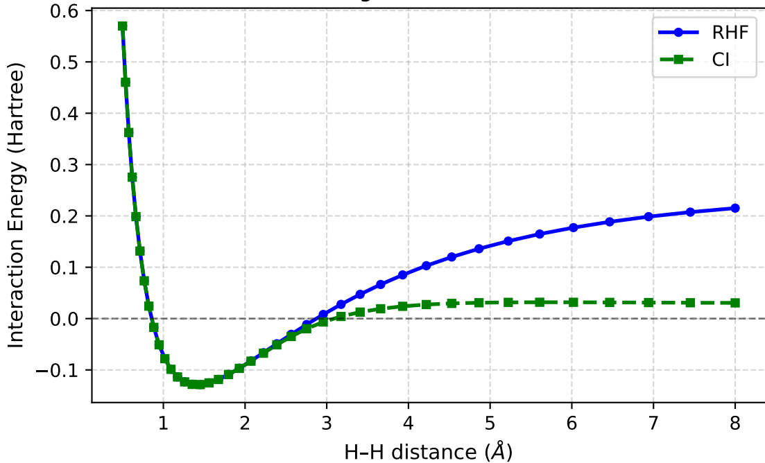
H 2 Binding Curve: E(\text{H}_2) - 2E(\text{H})
