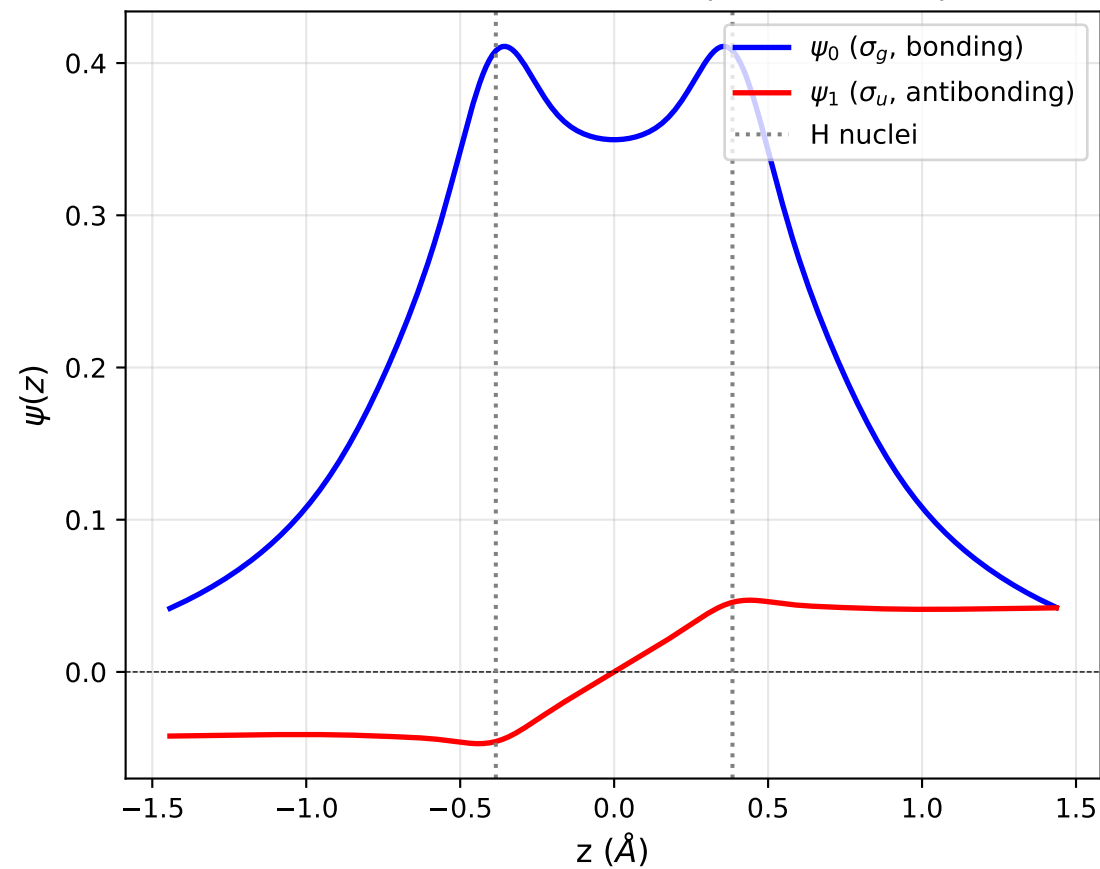
Orbital Wavefunctions ( R = 0.769 \text{ \AA} )
