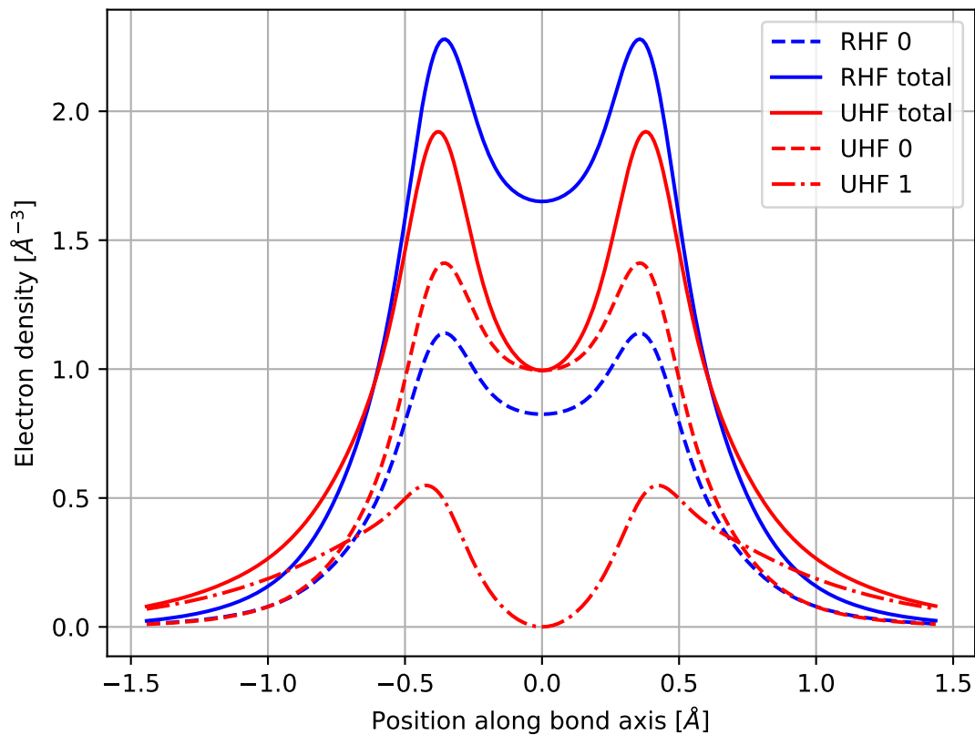
Densities at equilibrium R=0.769 \text{ \AA}
