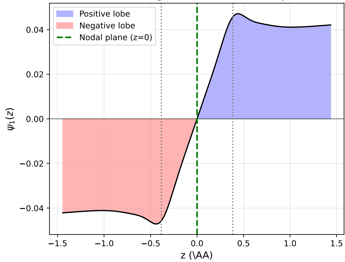
\sigma_u Antibonding Orbital (node at midpoint)
