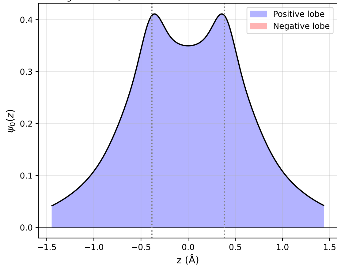
\sigma_g Bonding Orbital (no node between nuclei)
