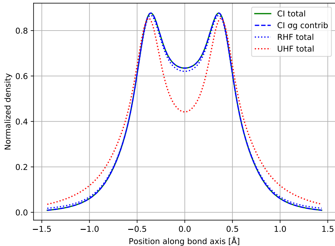
Equilibrium (CI from RHF orbitals) R=1.45 bohr
