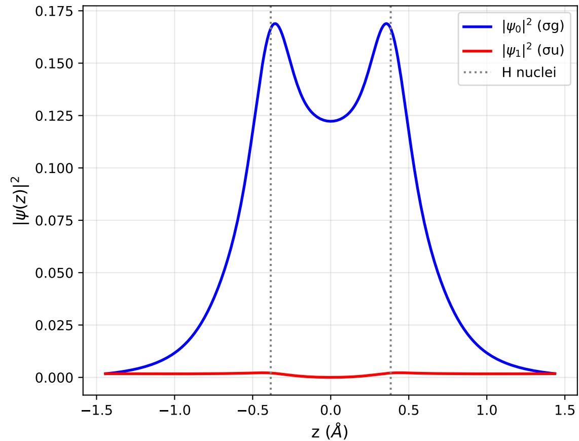
Orbital Densities
