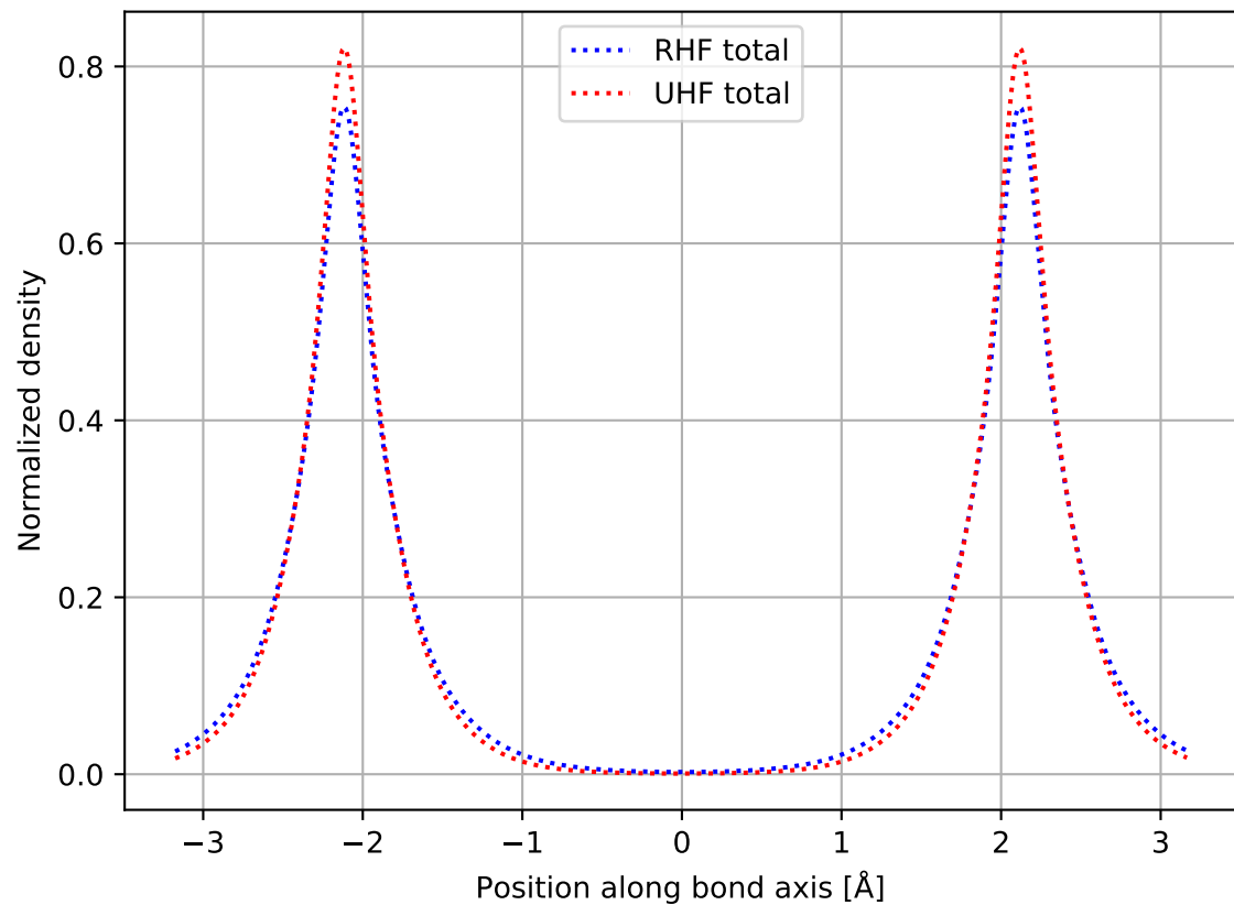
Max Separation (CI from UHF orbitals) R=8.00 bohr
