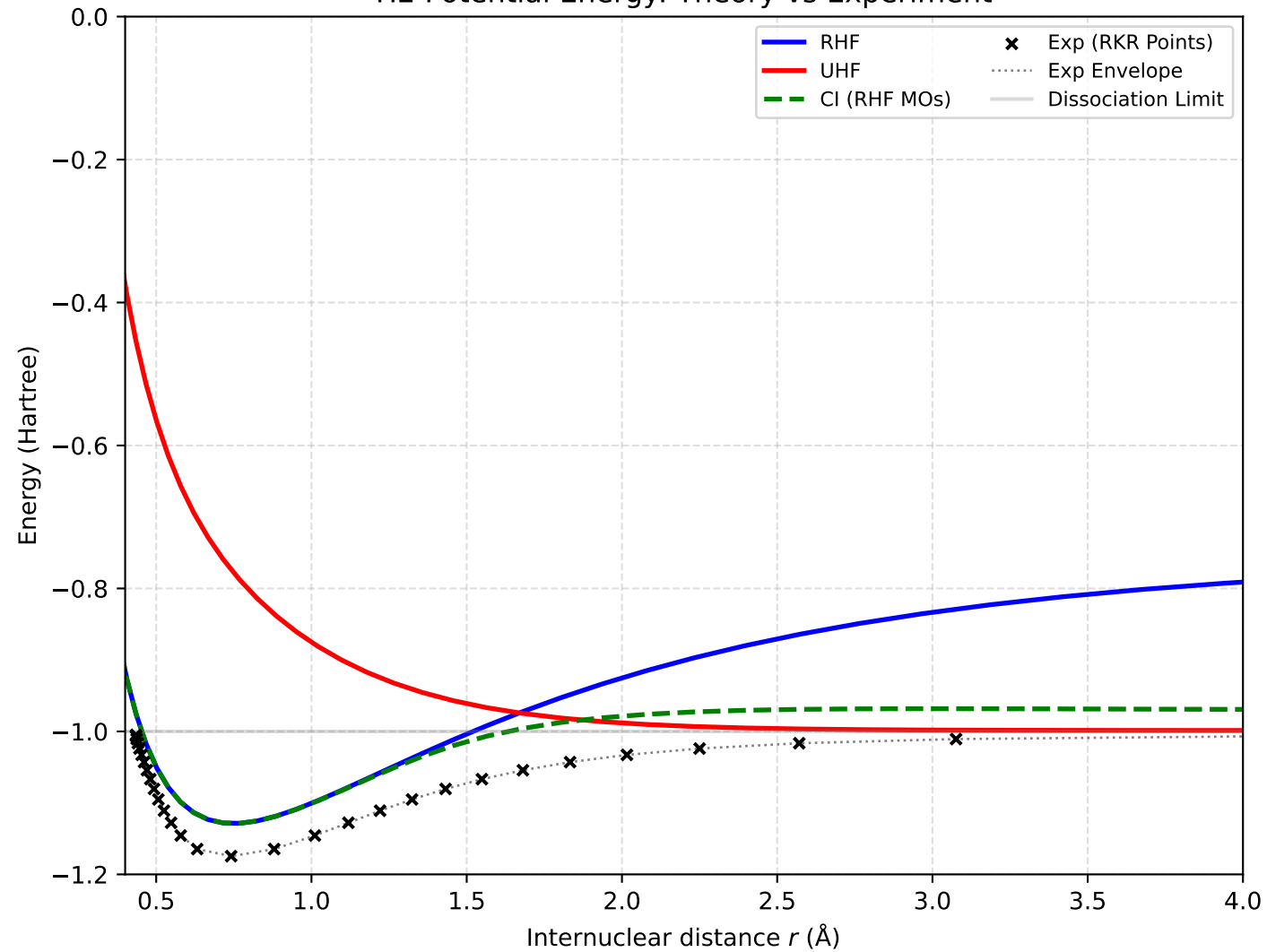
H2 Potential Energy: Theory vs Experiment
