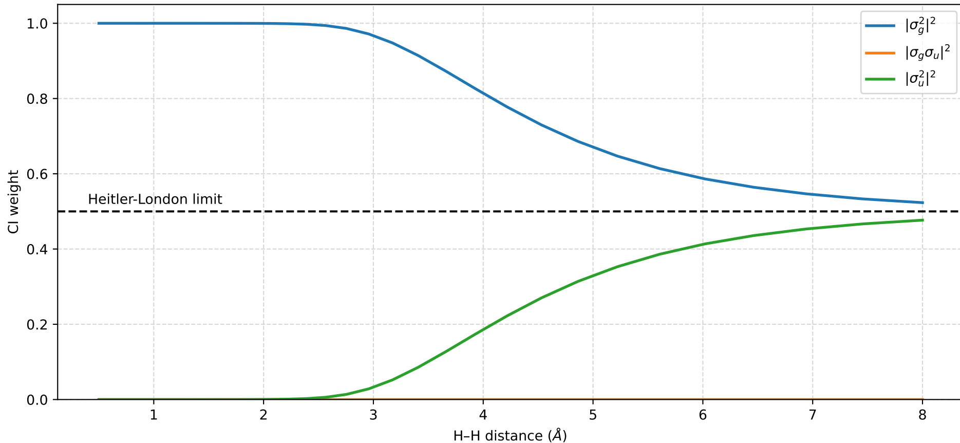
CI wavefunction composition vs H-H distance
