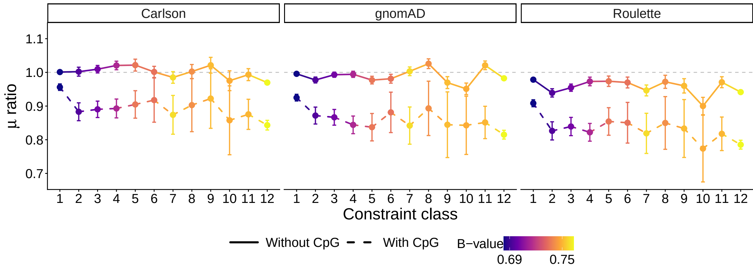
Ratios of mutation rates within (isolated) phastCons elements w.r.t. 1 kb background
