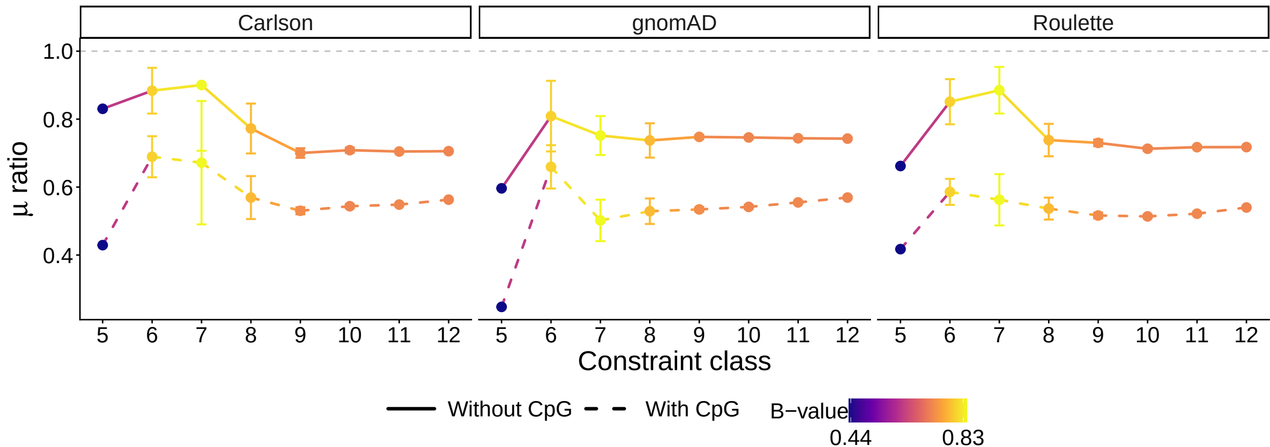
Ratios of mutation rates within (isolated) Benegas elements w.r.t. 1 kb background
