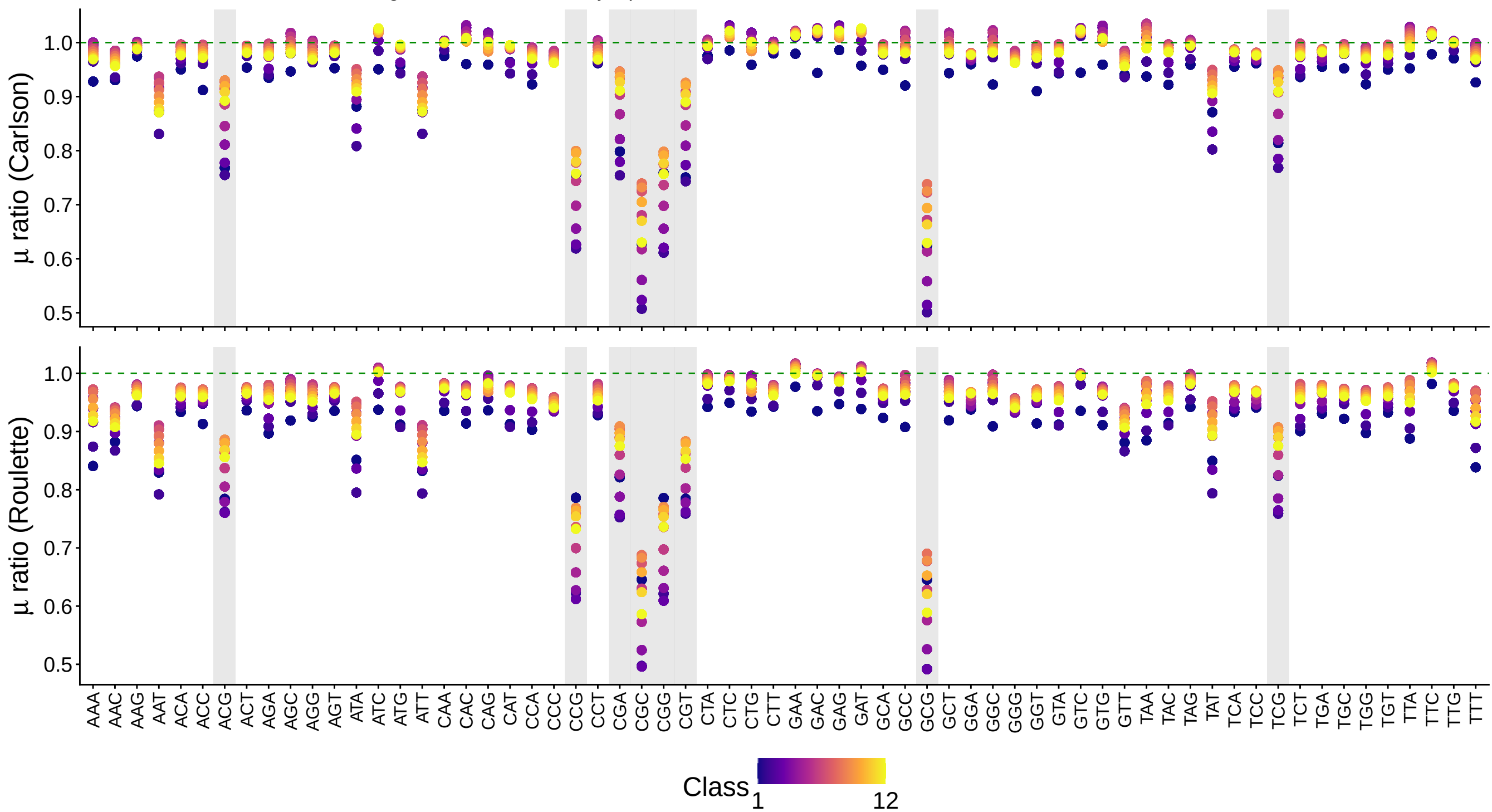
Ratios of mutation rates within Benegas elements stratified by triplet context
