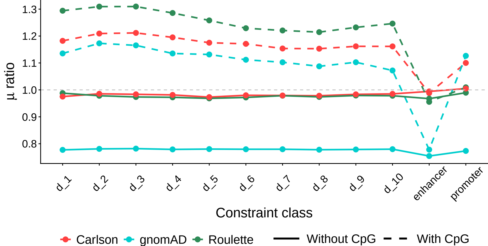
Ratios of mutation rates within functional elements w.r.t. genome-wide background
