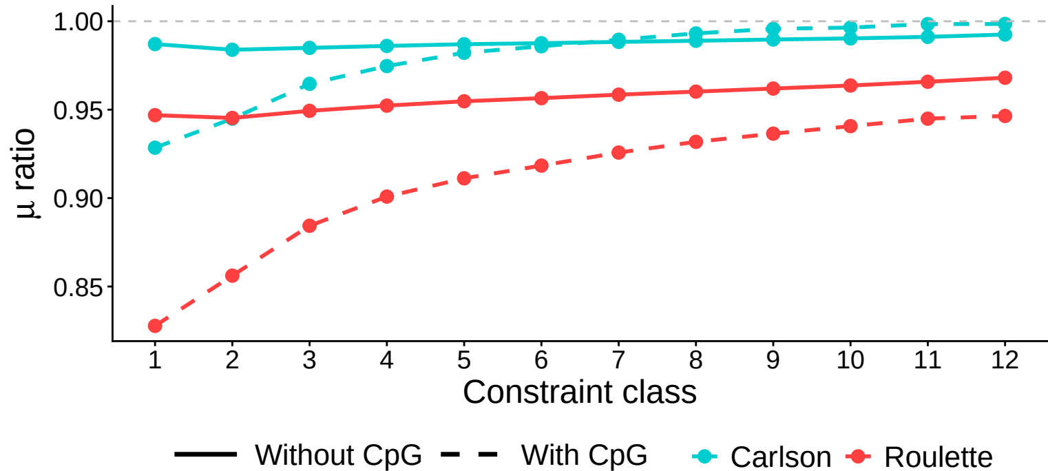
Ratios of mutation rates within phast elements w.r.t. genome-wide background
