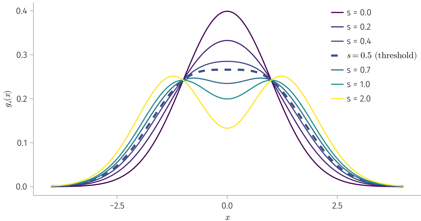
Density family across bimodality threshold
