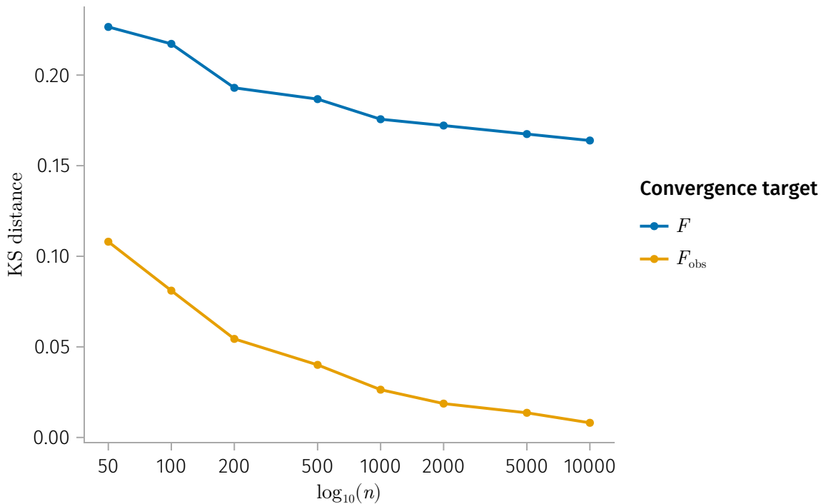
Prop 4: scores converge to F_{\text{obs}} , not F
