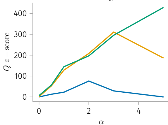
Normalized Q , \tau = 1.0
