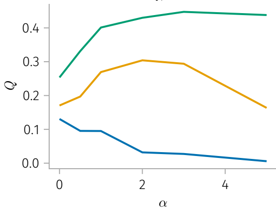
Raw Q , \tau = 1.0
