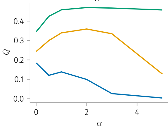
Raw Q , \tau = 3.0
