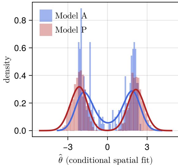
Recovered ideology distributions
