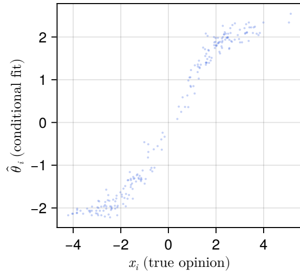
Model A : recovered \hat{\theta}_i
