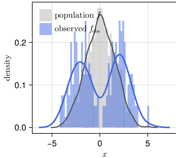
Model A : population vs observed
