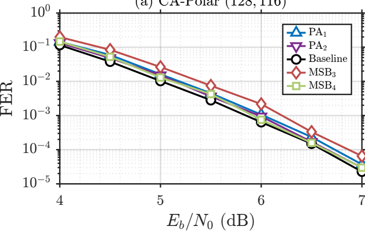
(a) CA-Polar (128, 116)
