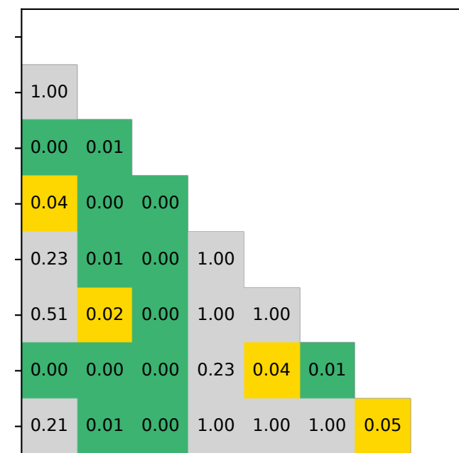
core - steric
