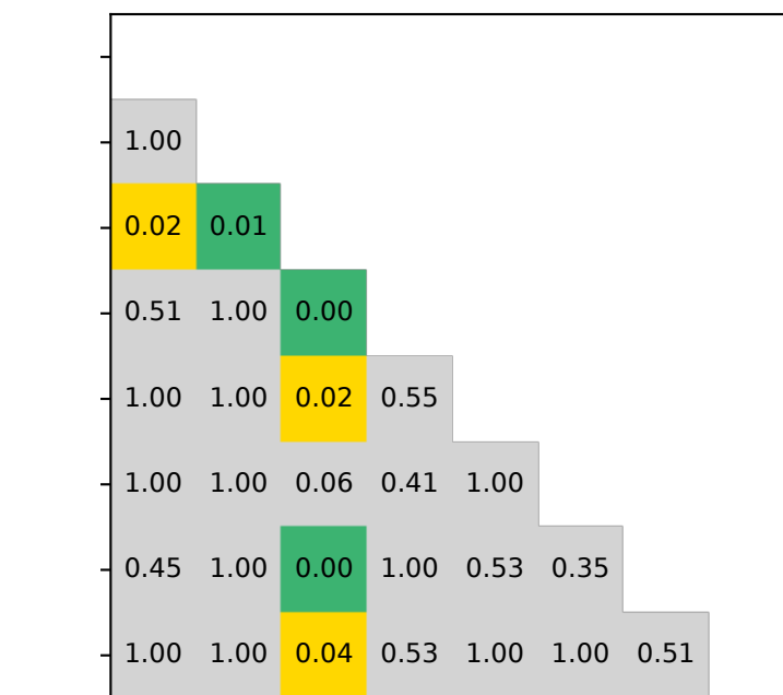
surface - steric
