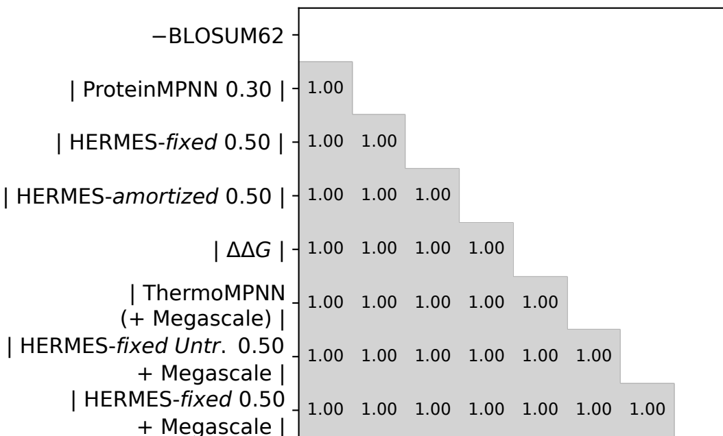
all - electronic
