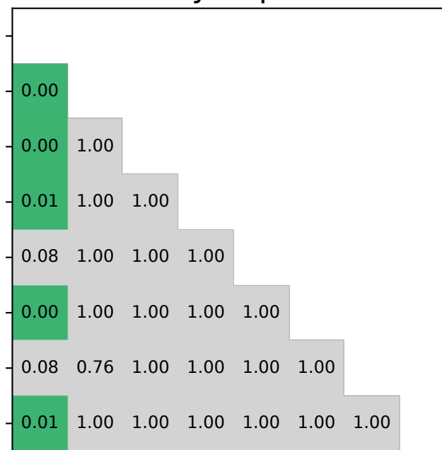
all - hydrophobic
