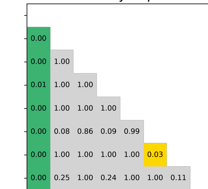
surface - hydrophobic
