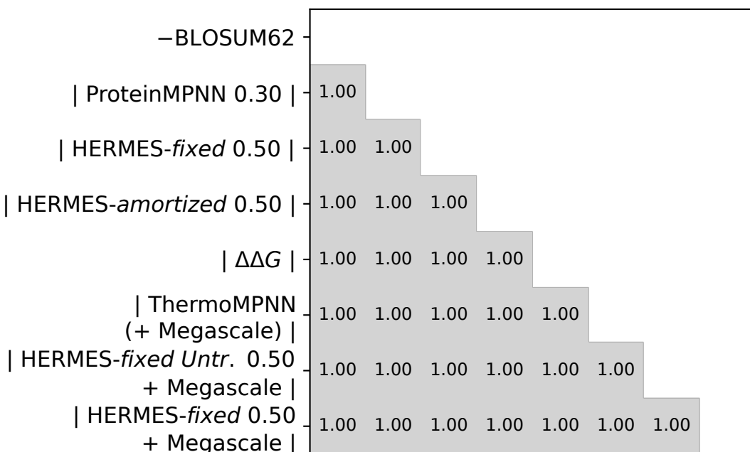
surface - electronic
