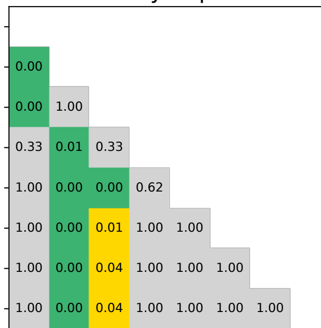
core - hydrophobic
