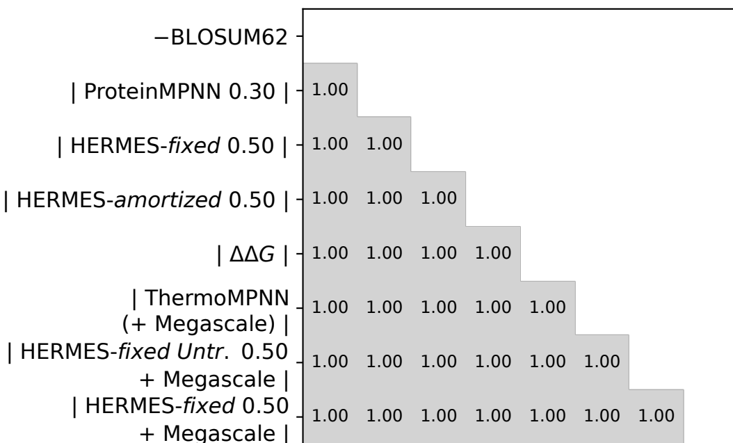
core - electronic
