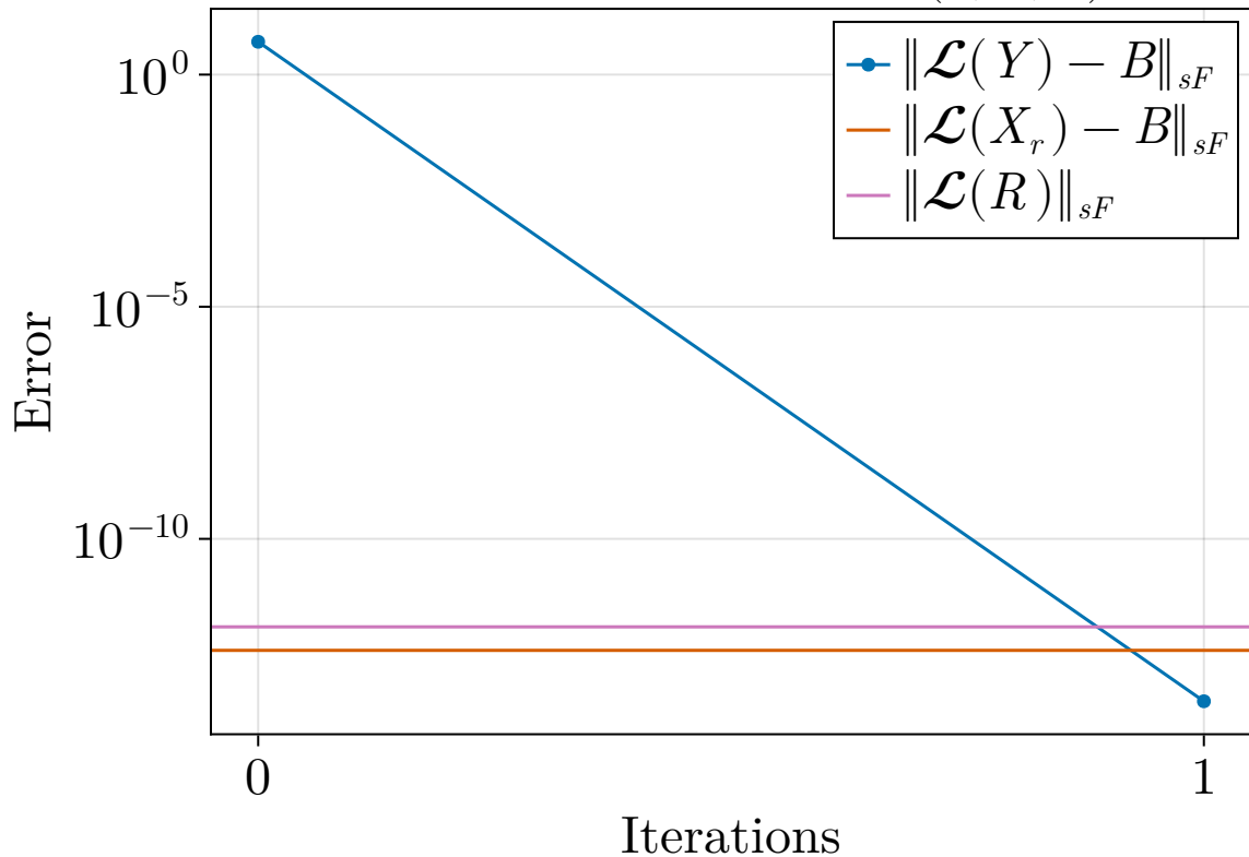
Multilinear rank of Y = (7, 7, 7)
