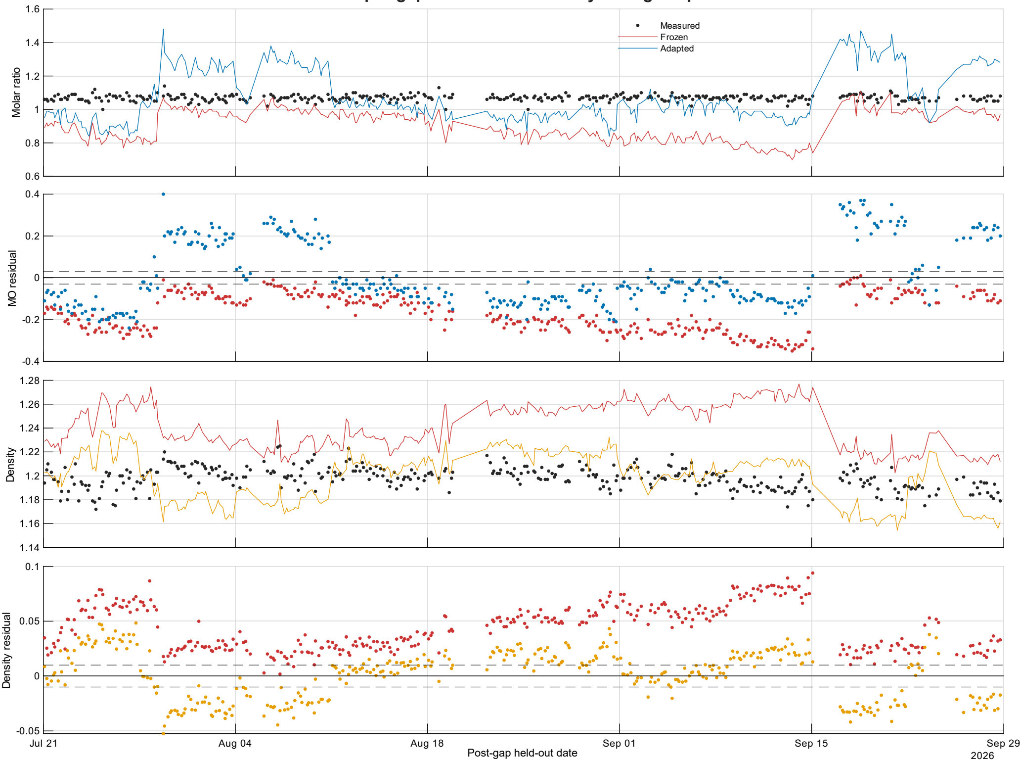
Frozen pre-gap model versus 14-day rolling adaptation
