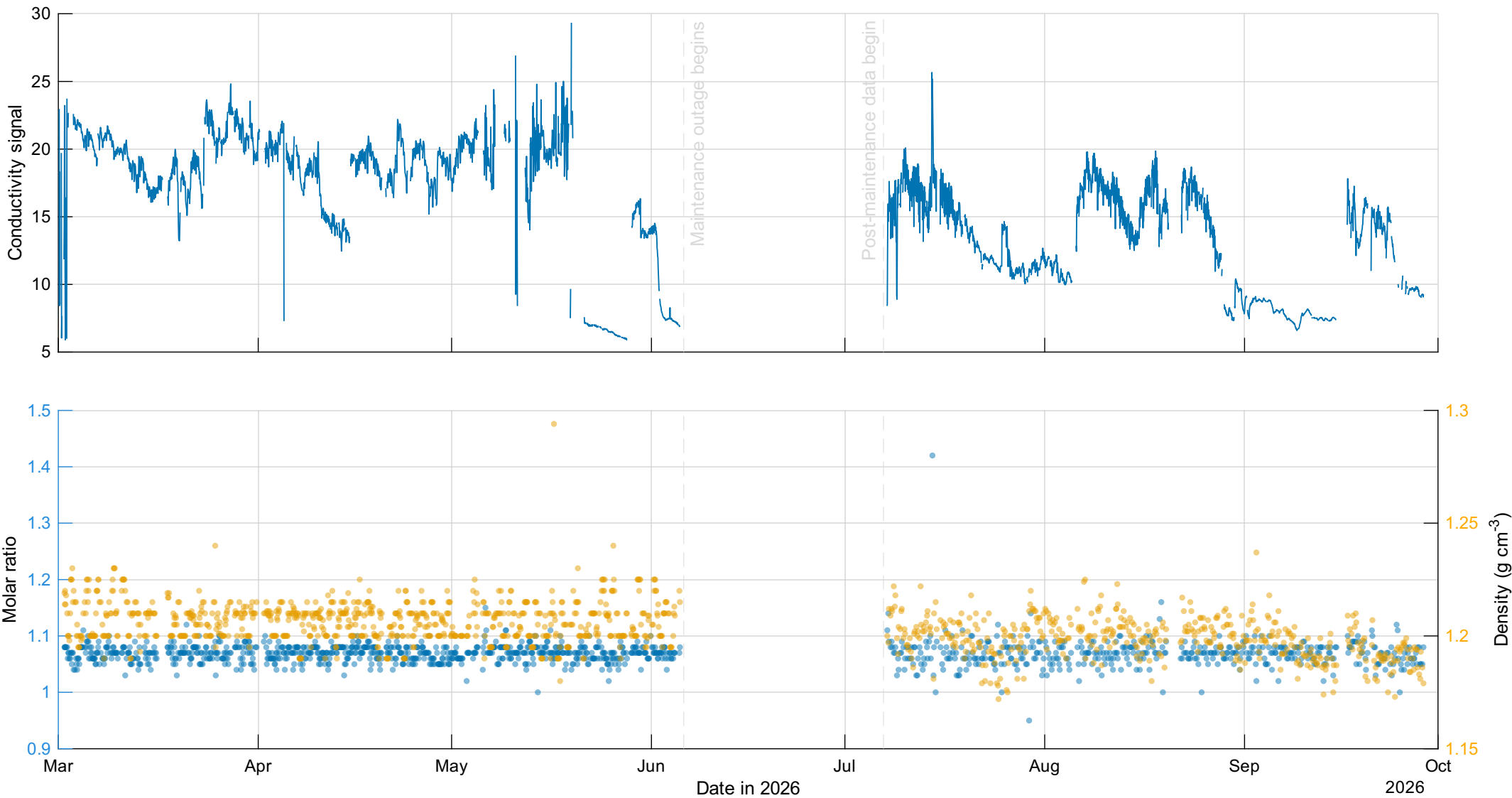
Extended process and laboratory coverage across the maintenance outage
